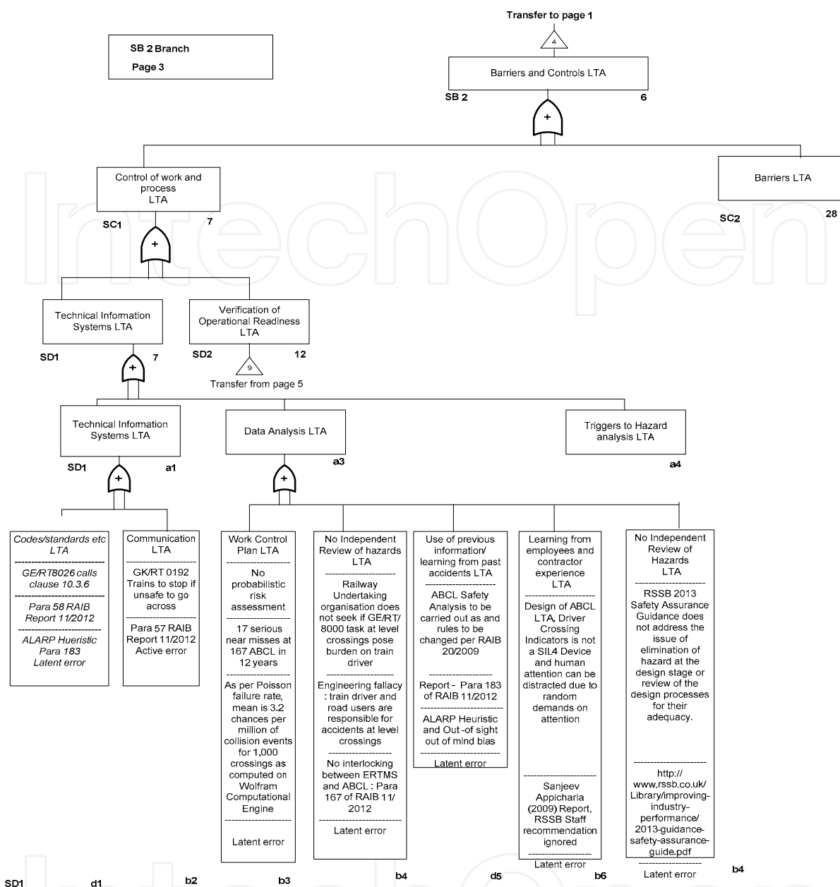
Figure 6. SIRS MORT SB2 Branch.
