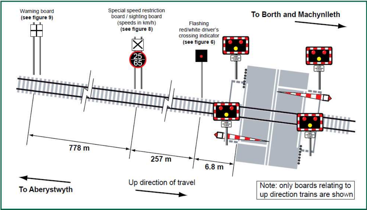
Figure 3. Schematic diagram of Llanbadarn ABCL.
