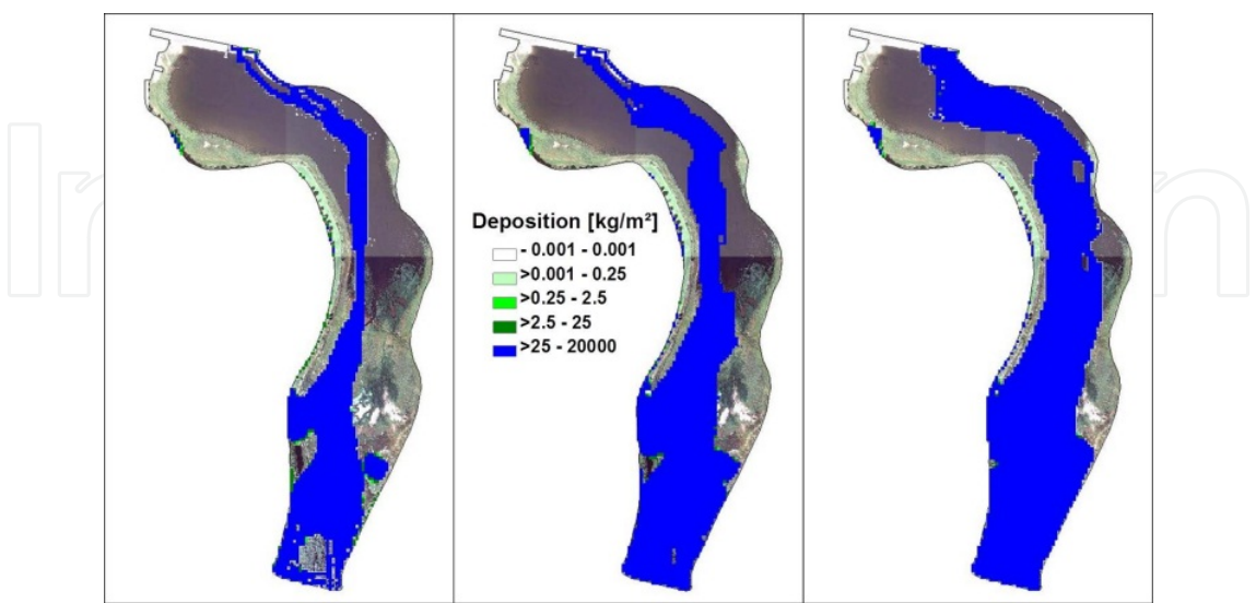
Figure 12. Siltation of the Baderitz Reservoir. Growing deposition areas after 1, 5, and 10 years.
