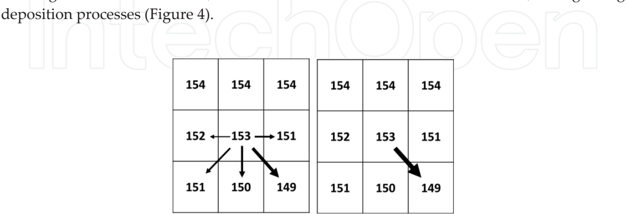
Figure 4. Multi-direction flow (FD8, left) and single direction flow (D8, right).
