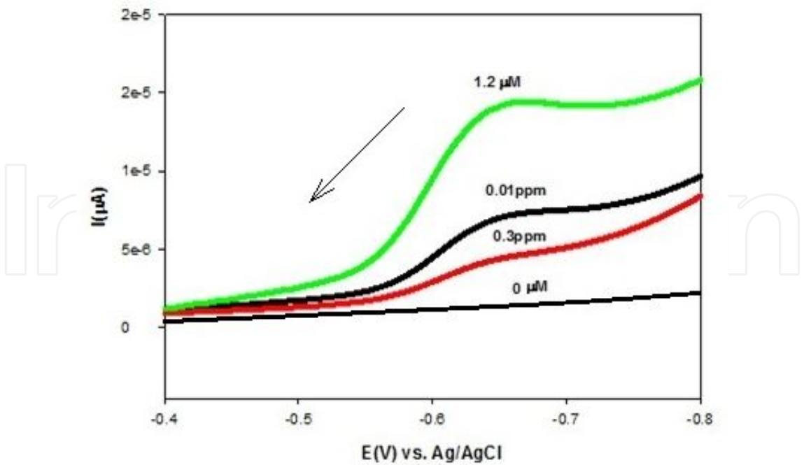
Figure 2. Results for the Pt/GO-PANI/HRP biosensor responses to an optimum 1.2 \mu\text{M} \text{H}_2\text{O}_2 substrate addition before incubation, and responses obtained after incubation in different carbaryl pesticide concentrations of 0.01 ppm ( n = 3 ; RSD = 4.67%) and 0.3 ppm ( n = 3 ; RSD = 6.92%), respectively.
