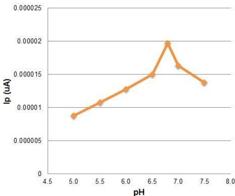
Figure 1. Results obtained for the optimisation of the pH of the Pt/GO-PANI/HRP biosensor evaluated in 0.1 M phosphate buffer, 0.1 M KCl solution with the addition of \text{H}_2\text{O}_2 as substrate.
