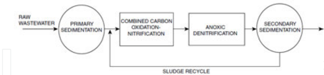
Figure 38. Nitrification/denitrification system for biological removal of nitrogen [3].
