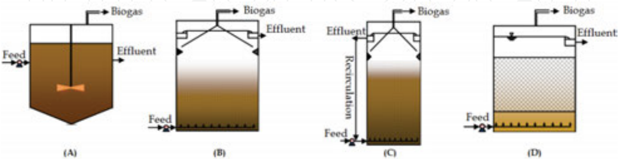
Figure 8. Most commonly used anaerobic reactor types: (A) Completely mixed anaerobic digester, (B) UASB reactor, (C) AFB or EGSR reactor, and (D) Upflow AF [8].
