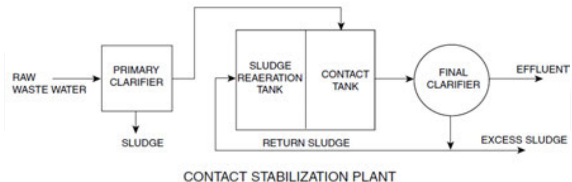
Figure 26. Contact stabilization plant [3].
