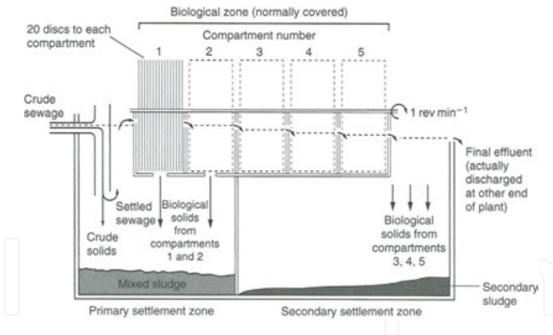
Figure 35. RBC system [1].
