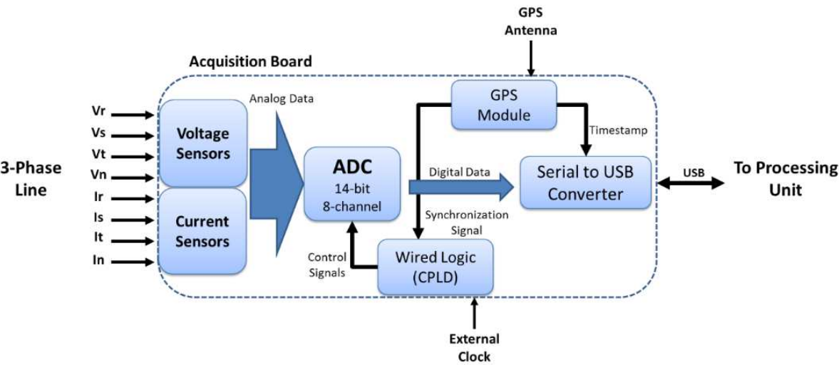
Figure 2. Acquisition board scheme.
