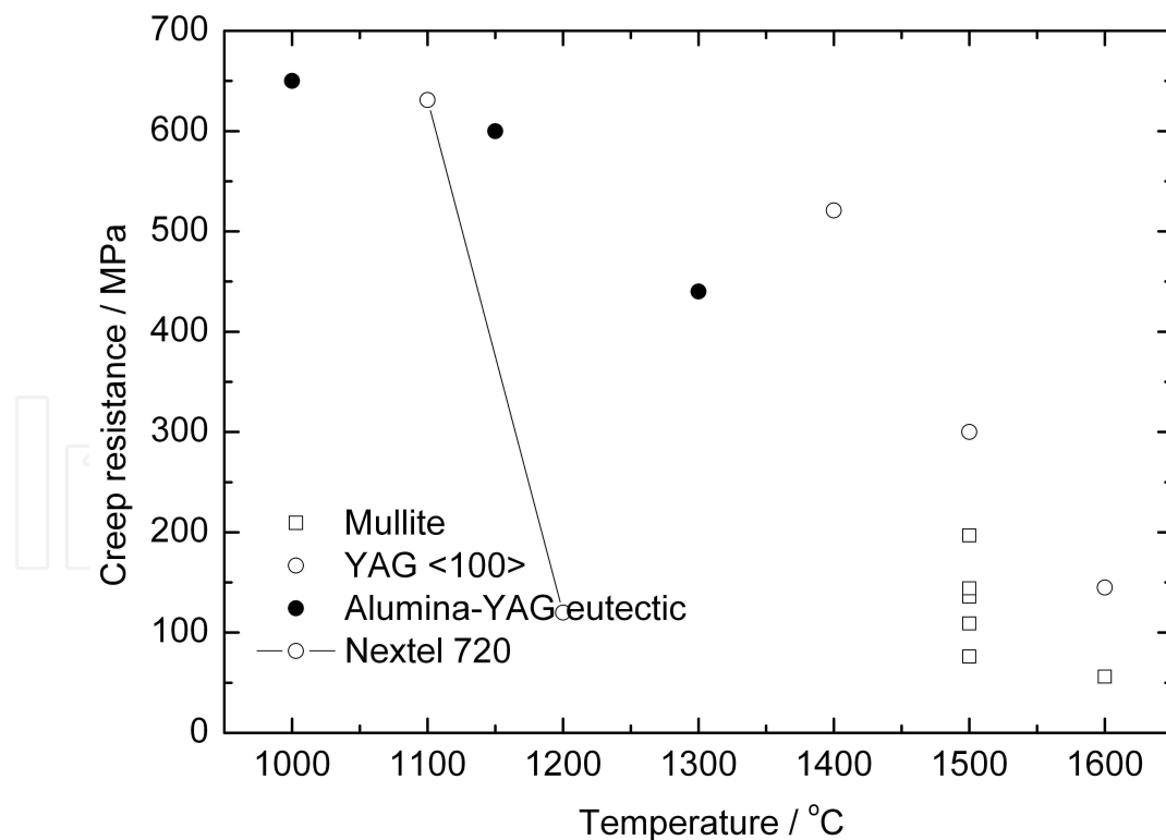
Figure 24. Creep resistance (stress to cause 1% creep strain for 100 h) of ICM-fibres in comparison with commercially available polycrystalline oxide fibres [47].
