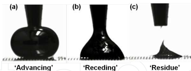
Figure 5. Advancing angle ( 160.5^\circ ), receding angle ( 77.9^\circ ), and residual state of the oxidized Galinstan ® on the micro pillar array with 75\ \mu\text{m} diameter and 100\ \mu\text{m} gap distance.
