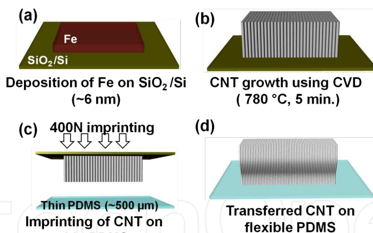
Figure 11. Fabrication sequence of the stretchable and bendable super-lyophobic CNT on PDMS sheet: (a) iron catalyst on Si, (b) vertically aligned CNT growth on Si, (c) imprinting CNT onto PDMS sheet, and (d) transferred CNT on PDMS sheet.
