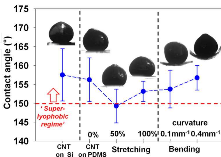
Figure 15. Static contact angle of \sim 7.8 \text{ }\mu\text{L} oxidized Galinstan® droplet on various surfaces.
