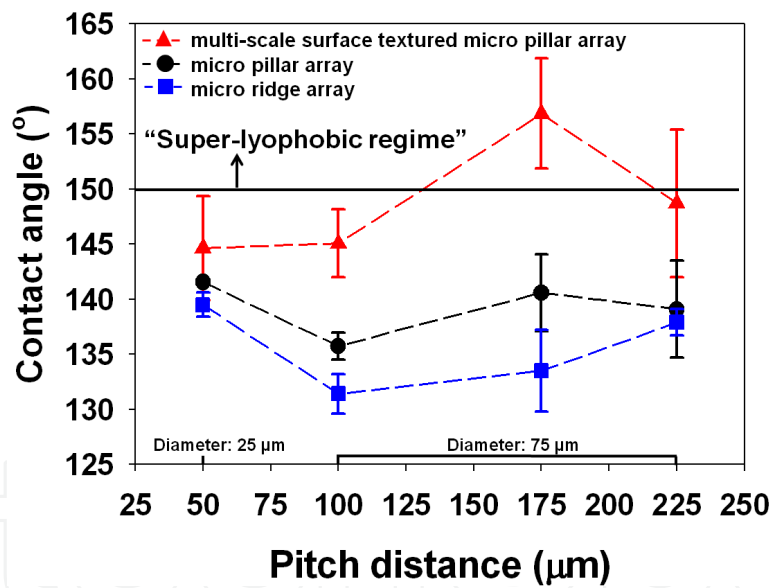
Figure 8. Contact angles of a 7.8 μL oxidized Galinstan ® droplet on a multi-scale surface textured micro pillar array, micro pillar, and ridge arrays.
