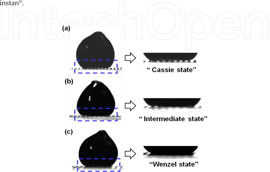
Figure 4. A 7.8 μL oxidized Galinstan® droplet on (a) 150 μm gap micro pillar array showing a non-wetting Cassie state, (b) 200 μm gap micro pillar array showing an intermediate transition state, and (c) 250 μm gap micro pillar array (no air pockets) showing a fully wetted Wenzel state. The diameter of all micro pillars is 75 μm.
