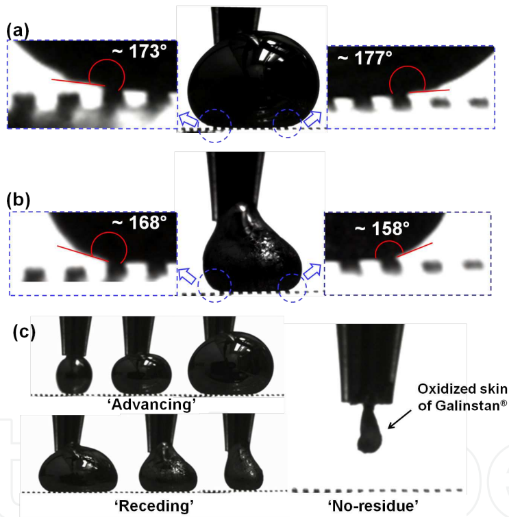
Figure 10. Optical images of an oxidized Galinstan® droplet on the multi-scale surface patterned PDMS micro pillar arrays (pitch distance 175 \mu\text{m} ) during dynamic contact angle test: (a) advancing contact angle ( \theta_{adv} = 175^\circ ), (b) receding contact angle ( \theta_{rec} = 163^\circ ), and (c) evidence of no-residue after receding from the surface.
