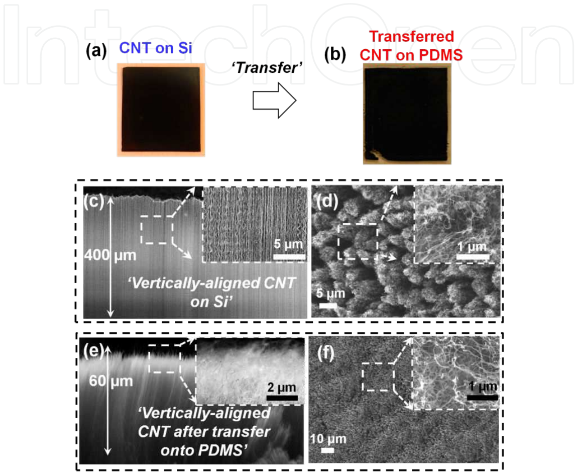
Figure 12. Optical and SEM images of CNT on Si and PDMS: optical images of (a) grown CNT on Si; (b) transferred CNT on PDMS sheet; (c) side-view SEM image of the vertically aligned CNT on Si; (d) top-view SEM image of the CNT showing micro/nano scale mixed morphology; (e) side-view SEM image of vertically aligned CNT after transfer onto the PDMS sheet; and (f) top-view SEM image of micro/nano surface morphology after the transfer.
