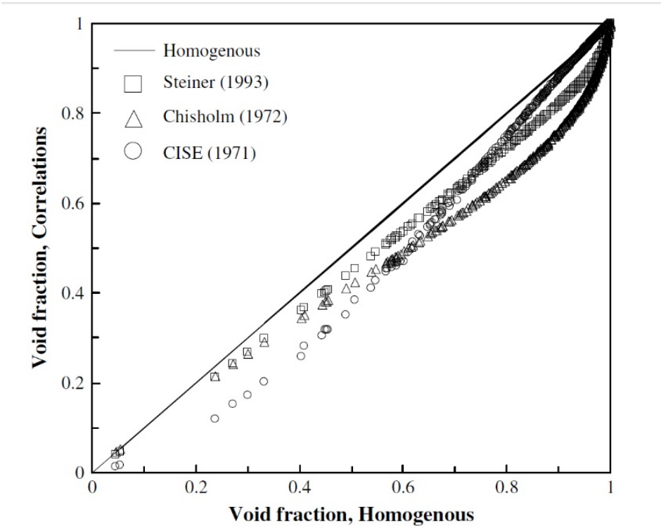
Figure 4. Void fraction comparison between the homogenous model and the existing correlations
