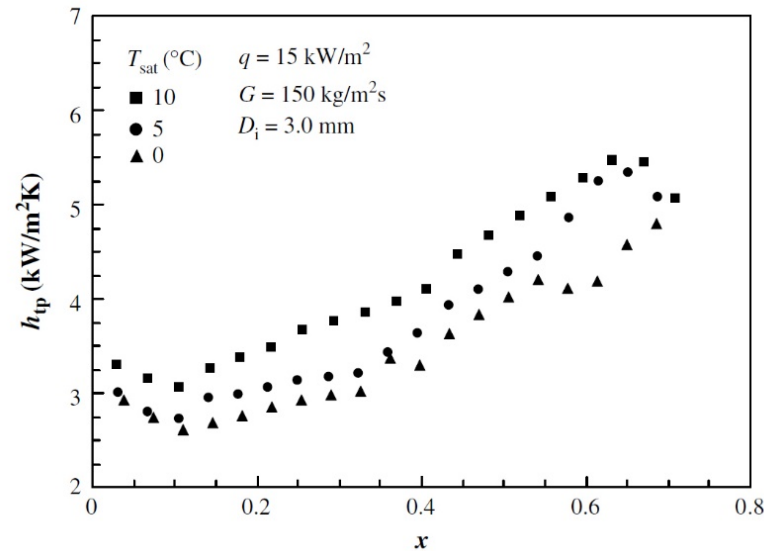
Figure 10. The effect of saturation temperature on heat transfer coefficient
