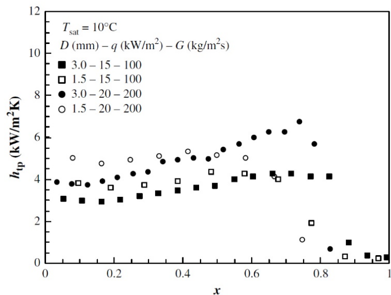
Figure 9. The effect of inner tube diameter on heat transfer coefficient
