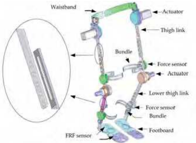
Fig. 2. Configuration of the robot suit
