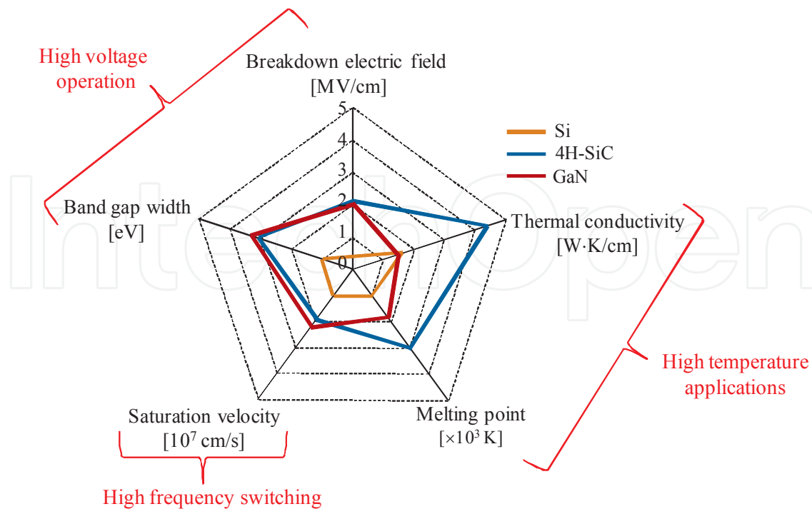
Figure 1. Summary of Si, SiC, and GaN relevant material properties.
