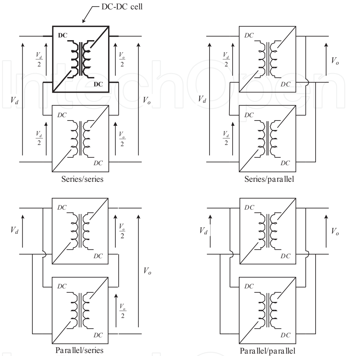
Figure 5. Possible associations between the DC-DC converters cells for N_{\text{cell}} = 2 .
