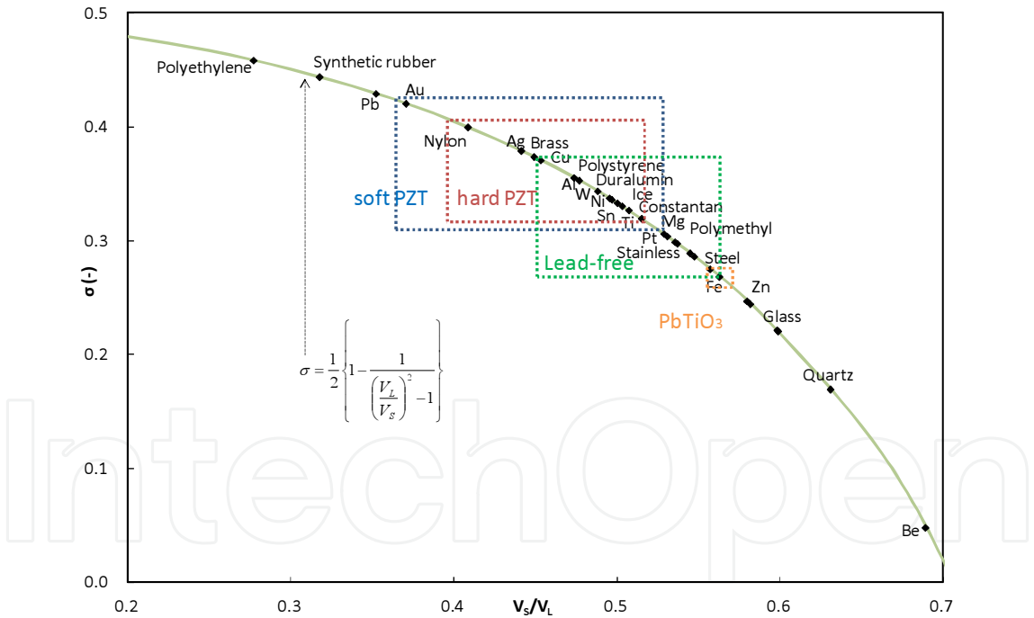
Figure 12. Relationship between ratio of sound velocities ( V_s/V_l ) and Poisson's ratio ( \sigma ) in solids including piezoelectric ceramics.
