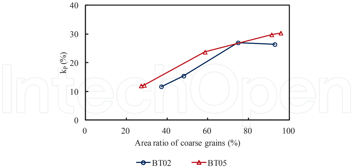
Figure 22. Planar coupling factor ( k_p ) vs. area ratio of coarse grains of black parts measured by an image-analyzing software program (WinRoof [39]).
