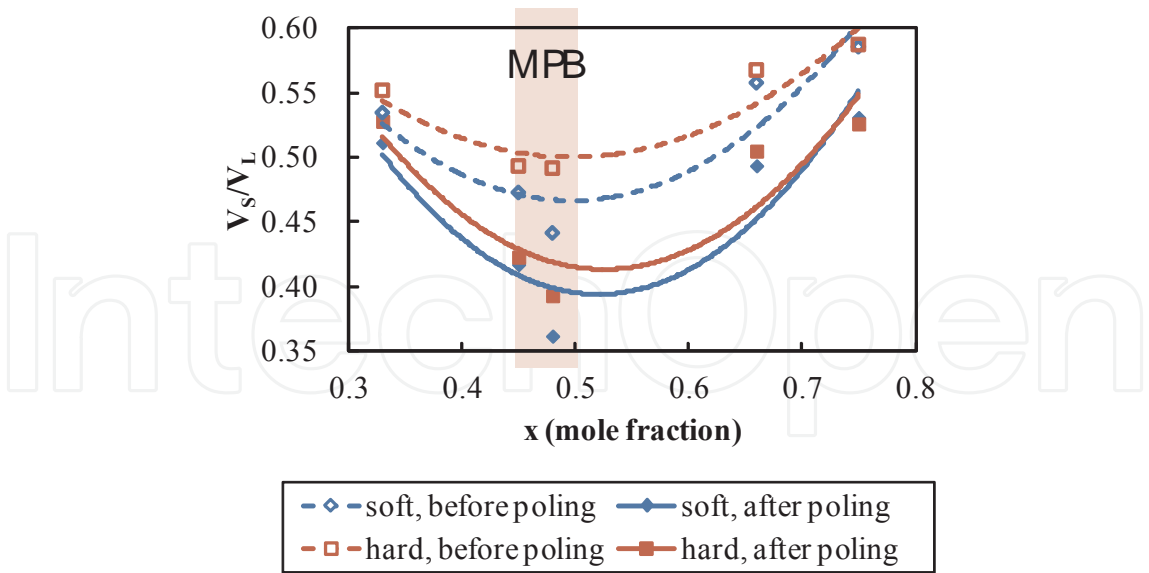
Figure 11. Composition x dependence of ratio of sound velocities ( V_s/V_l ) in 0.05\text{Pb}(\text{Sn}_{0.5}\text{Sb}_{0.5})\text{O}_3-(0.95-x)\text{PbTiO}_3-x\text{PbZrO}_3 ( x = 0.33, 0.45, 0.48, 0.66, 0.75 ) with (hard PZT) and without 0.4 wt% \text{MnO}_2 (soft PZT) ceramics before and after poling.
