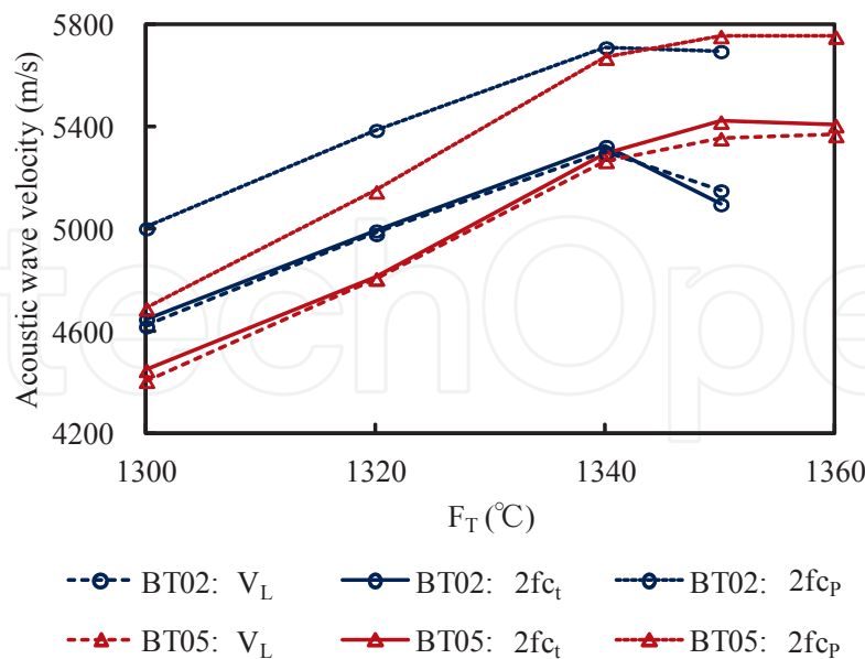
Figure 15. Comparison between longitudinal wave velocity ( V_L ), 2fc_t and 2fc_p , which are twice the frequency constants of fc_t for the thickness mode and fc_p for the radial mode on disks in BT02 and BT05 ceramics after DC poling; 2fc_t and 2fc_p correspond to acoustic wave velocities.
