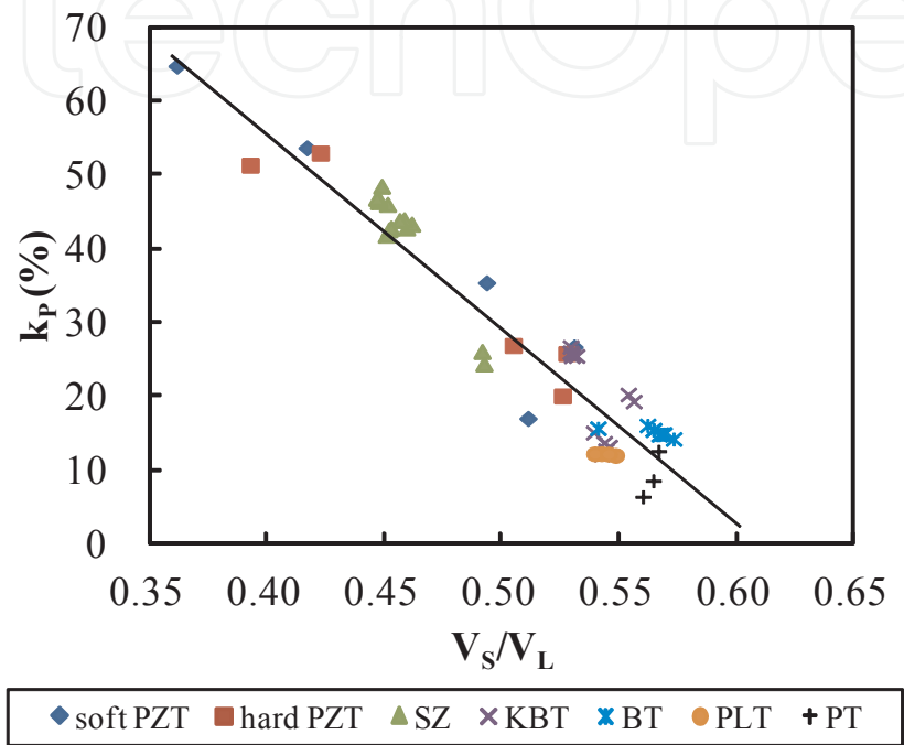
Figure 6. Relationship between ratio of sound velocities ( V_s/V_L ) and planar coupling factor ( k_p ) in lead-free and lead-containing ceramics.
