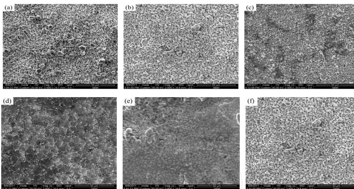
Figure 9. Representative scanning electron micrographs of Zn-Ti alloys electrodeposited on mild steel from \text{ZnCl}_2 -urea (molar ratio 10:1) containing 0.43 \text{ mol L}^{-1} \text{ TiCl}_4 (a) and with 1.67 \text{ mol L}^{-1} following additives: (b) LiCl, (c) NaCl, (d) KCl, (e) \text{NH}_4\text{Cl} and (f) TMAC.
