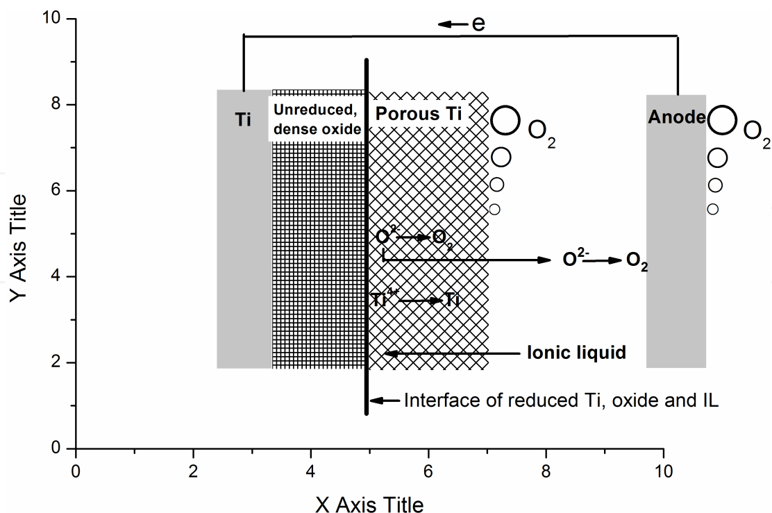
Figure 4. Model for the reduction process of oxides film on titanium foil in Lewis basic AlCl_3 -BMIC ionic liquid. [Ref. 13]
