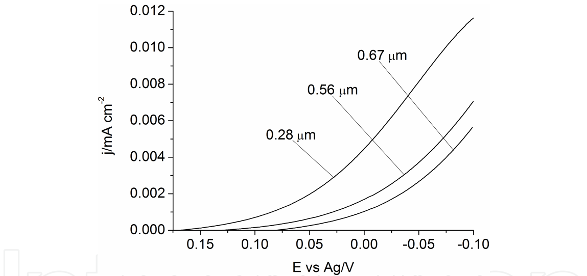
Figure 2. Cathode polarization curves for oxidized Ti foils with different thickness of titanium oxide film in Lewis basic \text{AlCl}_3\text{-BMIC} at 343\text{ K} and 5\text{ mV s}^{-1} . [Ref.12]
