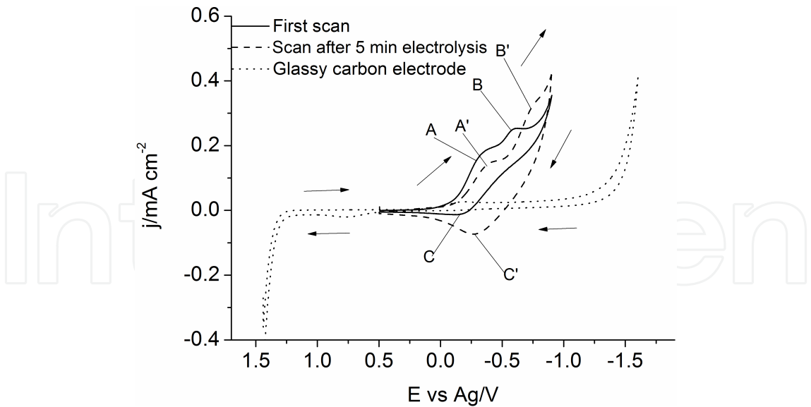
Figure 1. Cyclic voltammograms of oxidized Ti foil and glassy carbon electrode in Lewis basic \text{AlCl}_3\text{-BMIC} obtained at 50\text{ mV s}^{-1} and 343\text{ K} . [Ref.12]
