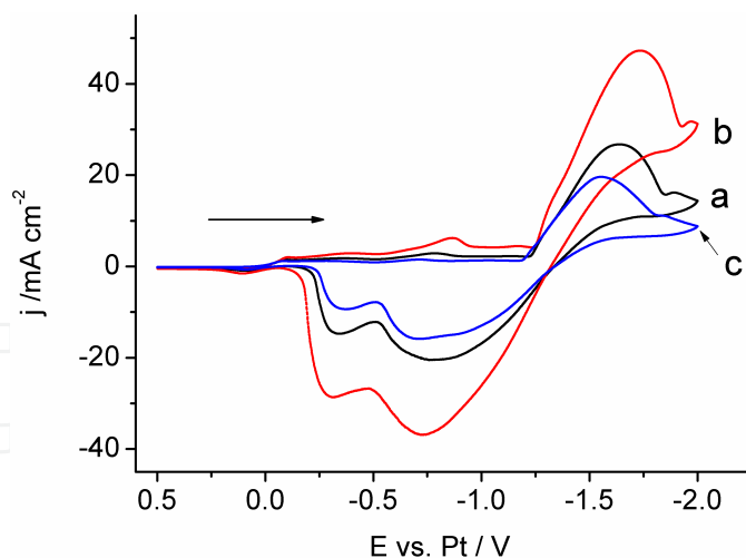
Figure 5. Cyclic voltammograms obtained at glassy carbon electrode at 50 \text{ mV s}^{-1} in \text{AlCl}_3\text{-BMIC-TiCl}_4 (molar ratio 2:1:0.037) (a) and with the following additives: (b) 0.25 \text{ mol dm}^{-3} toluene and (c) 0.25 \text{ mol dm}^{-3} \text{NH}_4\text{Cl}
