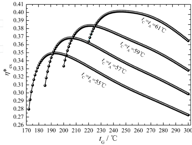
Figure 26. Effects of t_G on \eta_{\text{ex}}^* for t_G = 170\text{--}300^\circ\text{C} with t_A = t_C = 55^\circ\text{C} , 57^\circ\text{C} , 59^\circ\text{C} , or 61^\circ\text{C} and t_E = -10^\circ\text{C} [25].
