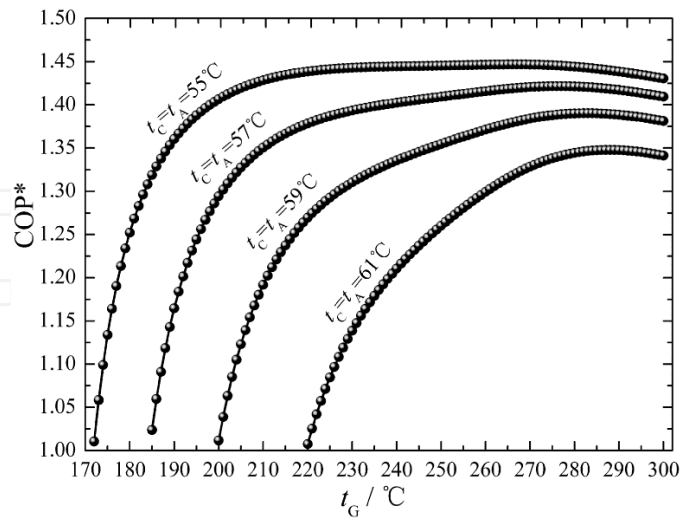
Figure 25. Effects of t_G on the \text{COP}^* for t_G = 170\text{--}300\text{ }^{\circ}\text{C} with t_A = t_C = 55\text{ }^{\circ}\text{C} , 57\text{ }^{\circ}\text{C} , 59\text{ }^{\circ}\text{C} , or 61\text{ }^{\circ}\text{C} and t_E = -10\text{ }^{\circ}\text{C} [25].
