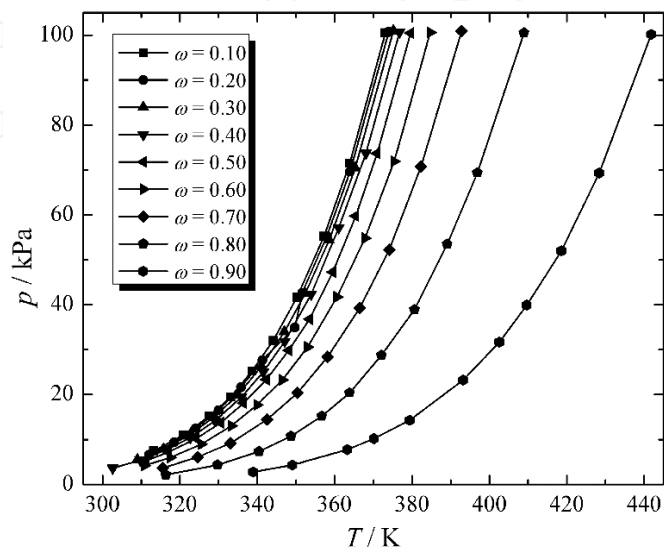
Figure 5. Vapor pressures of [dmIm]DMP-H 2 O.
