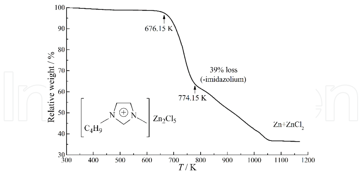
Figure 15. Thermogravimetric (TG) scan results for [bmim]Zn 2 Cl 5 .
