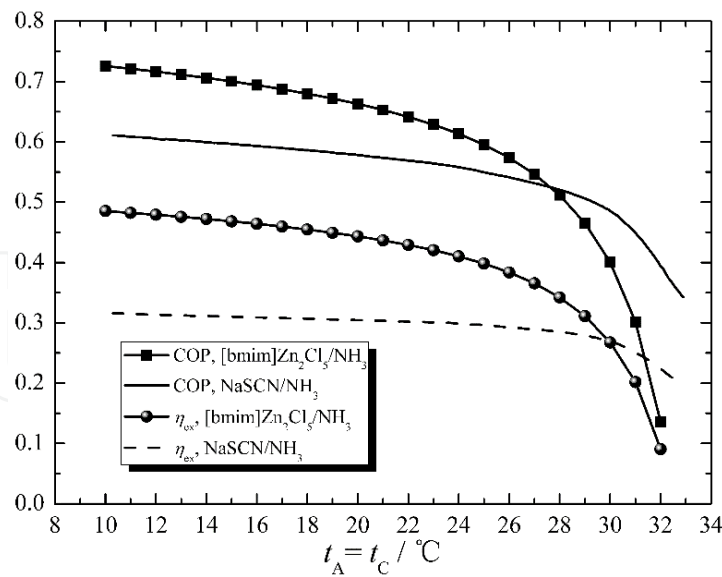
Figure 22. Variations in the COP and \eta_{\text{ex}} of [bmim] \text{Zn}_2\text{Cl}_5/\text{NH}_3 absorption refrigeration with varying t_A and t_C for t_G = 90\text{ }^\circ\text{C} and t_E = -10\text{ }^\circ\text{C} [25].
