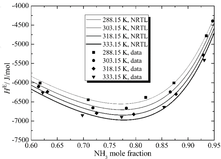
Figure 17. T - x - H^E diagram of [\text{bmim}]\text{Zn}_2\text{Cl}_5/\text{NH}_3 for T = 288.15\text{--}333.15\text{ K} .
