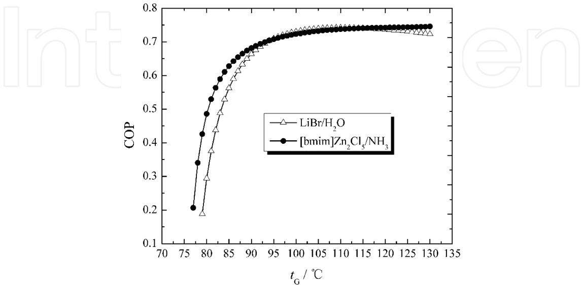
Figure 28. Effects of t_G on the COP for t_G = 75\text{--}130\text{ }^\circ\text{C} with t_A = 35^\circ\text{C} , t_C = 40\text{ }^\circ\text{C} , and t_E = 5\text{ }^\circ\text{C} .
