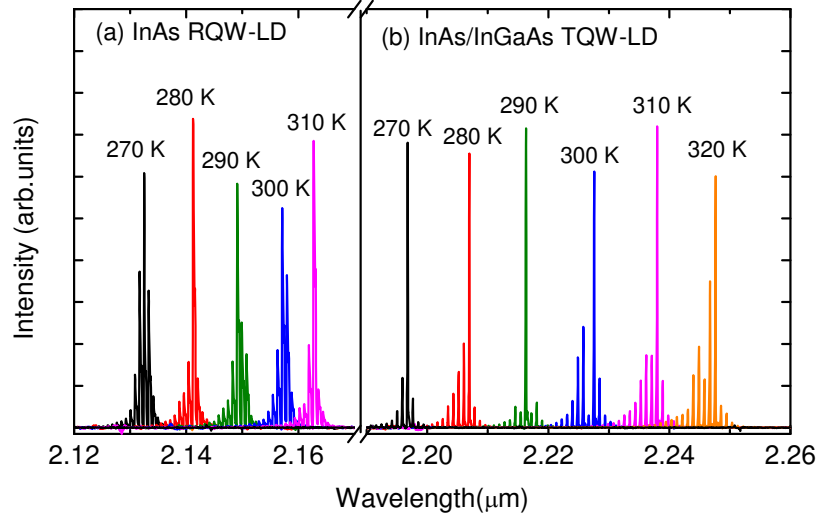
Figure 8. Lasing spectra of (a) rectangular QW laser and (b) triangular QW laser around 2.2 \mu\text{m} at various temperatures under CW driving condition.
