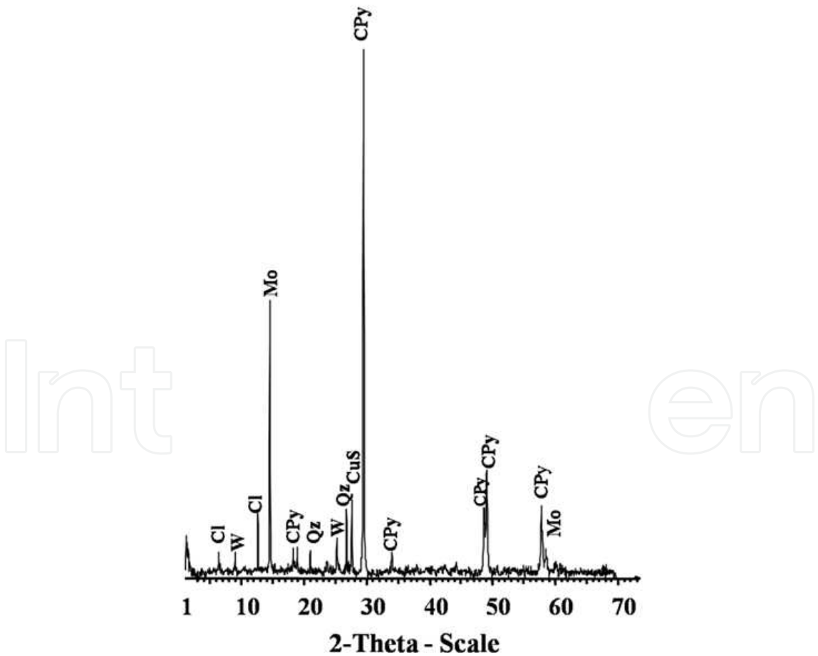
Figure 8. X-ray diffraction spectra for chalcopyrite of sample before the bioleaching process (CPy, chalcopyrite; Qz, quartz; Mo, molybdenite; W, wollastonite; Cl, chlorite; CuS, covellite).
