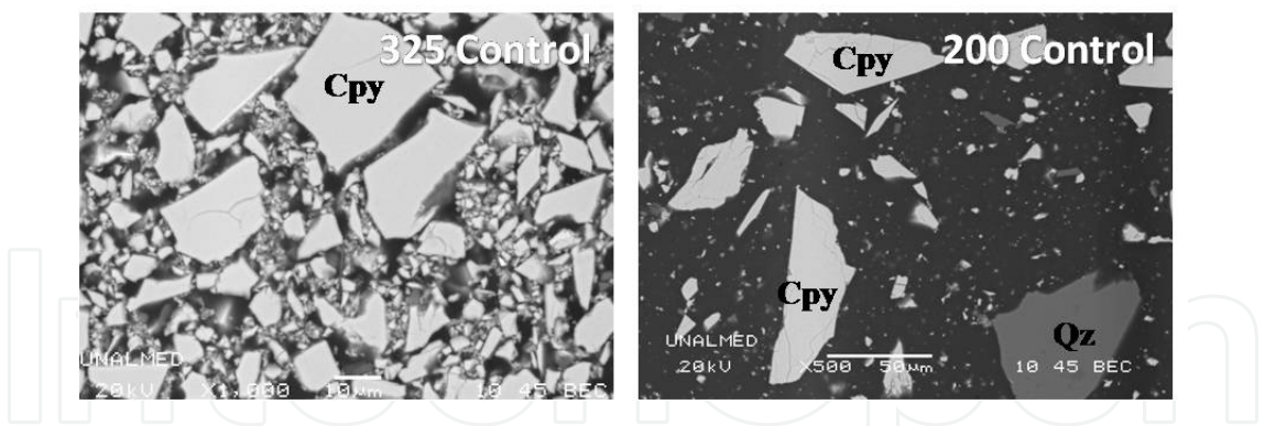
Figure 5. Scanning electron microscopy micrographs of uninoculated residues after chalcopyrite bioleaching. Cpy, chalcopyrite; Qz, quartz. After 30 days.
