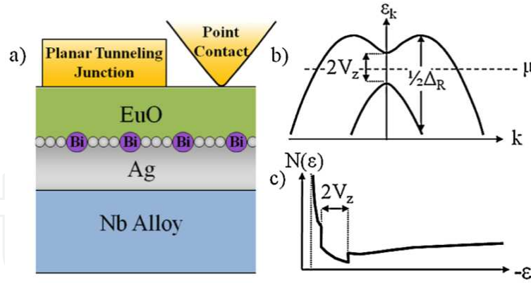
Figure 5. The proposed sample layout for the heavy-metal-based Majorana fermion creation [34]. (a) Ag(111) surface with 1/3 monolayer of Bi coverage in the (\sqrt{3} \times \sqrt{3}) R30^\circ reconstruction. Superconducting proximity from an s-wave superconductor (Nb alloy), and magnetic proximity from a magnetic insulator (EuO), together create a topological superconductor channel on the system. (b) Electrons confined on the metal surface experience strong Rashba spin-orbit coupling and form two parabolas crossing at k=0 . The gap of 2V_z comes from the exchange fields from EuO, and the chemical potential \mu of the system needs to be tuned to the mid-gap. (c) Potential verification of the surface states through tunnelling spectrum, where one should see a dip corresponding to the opening of the exchange gap and a van Hove singularity corresponding to the very top of the Rashba bands.
