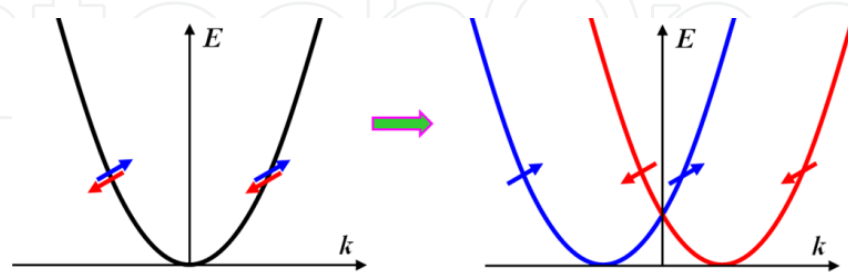
Figure 3. Illustration of a Rashba type spin-orbit splitting. Left: a typical parabolic “free” electron band with two-fold spin degeneracy. Right: In the presence of Rashba spin-orbit coupling, moving electrons feel an effective magnetic field on their rest frame, and the two spin channels are therefore split in energy. The effect is linear with respect to the wave vector k , and opposite for the two types of spins. Therefore, the Rashba spin-orbit coupling adds a linear component to the quadratic function, creating a uniform shift of the parabolas from the origin but in opposite directions for the opposite spin channels.
