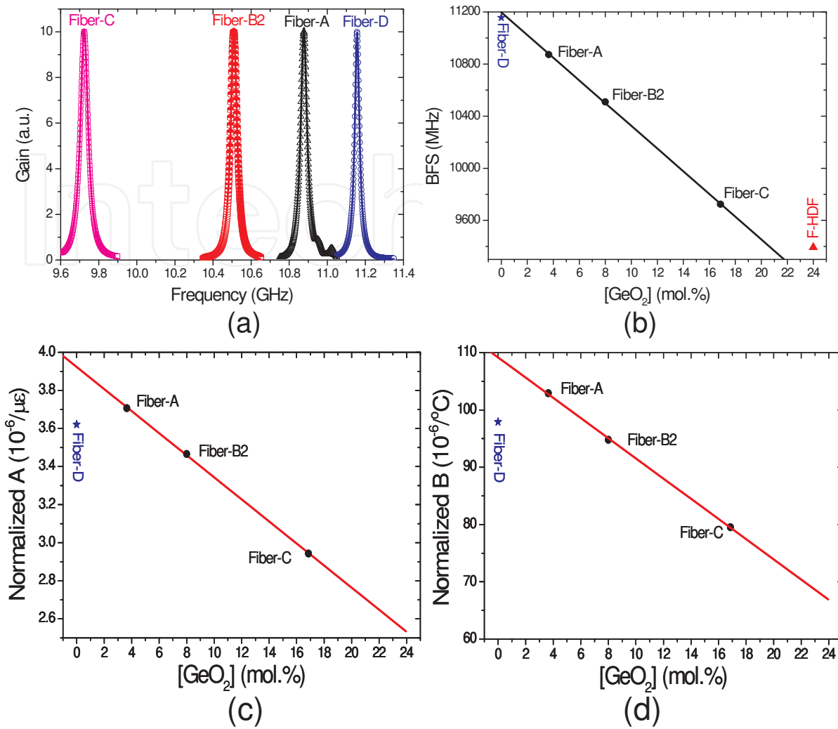
Figure 11. (a) BGS, (b) BFS, (c) normalized strain coefficient, and (d) normalized temperature coefficients in silica optical fibers with different \text{GeO}_2 concentration. (After Ref. [49]. © 2008 OSA/IEEE.)
