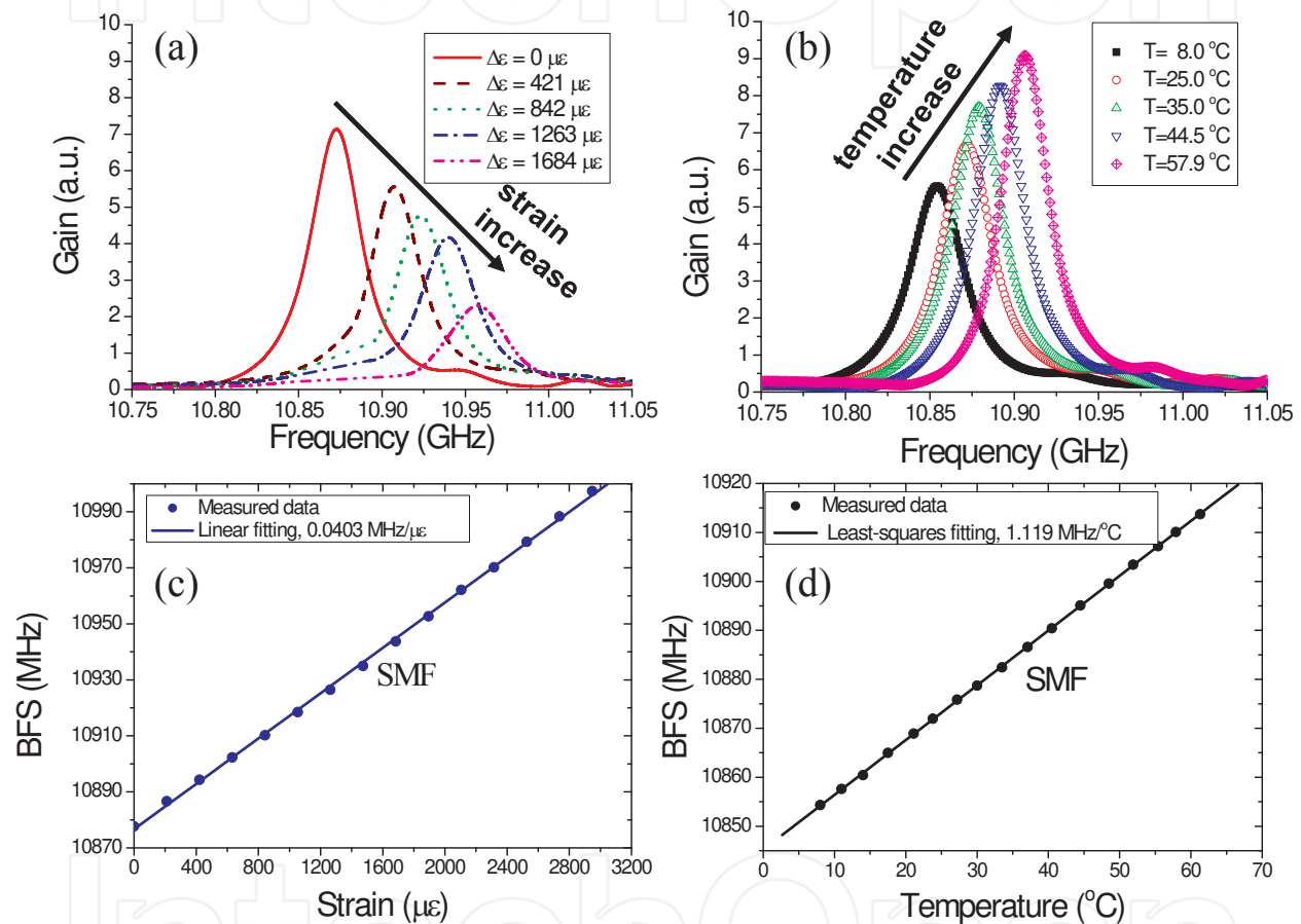
Figure 10. (a) Strain and (b) temperature dependences of BGS in SMF; (c) Strain and (d) temperature dependences of Brillouin frequency shift v_B in SMF.
