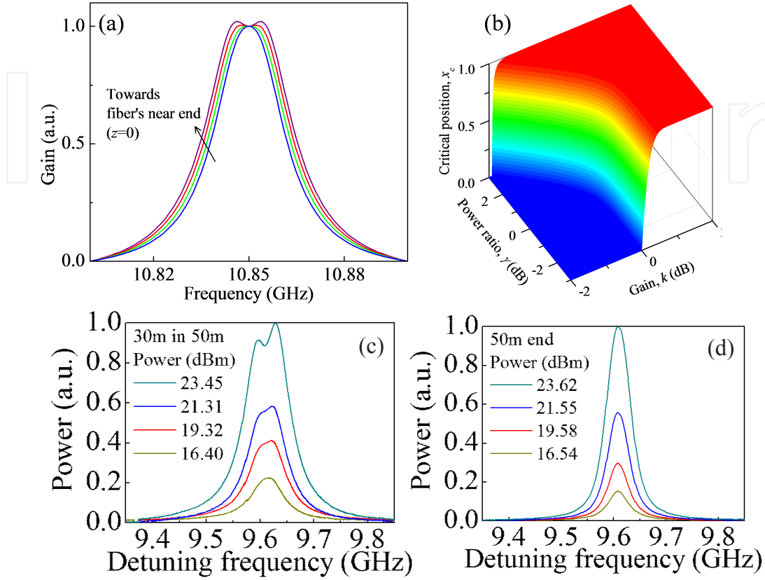
Figure 8. (a) Simulated BGS at different positions in the fiber. (b) Critical position x_c determined by the normalized gain k and injected power ratio \gamma . The critical positions divide the fiber into two parts with and without the spectral hole burning phenomenon. Measured BGS in the middle (c) or at the end (d) of a 50-m-long fiber. (after Ref. [42]; © 2014 JJAP.)
