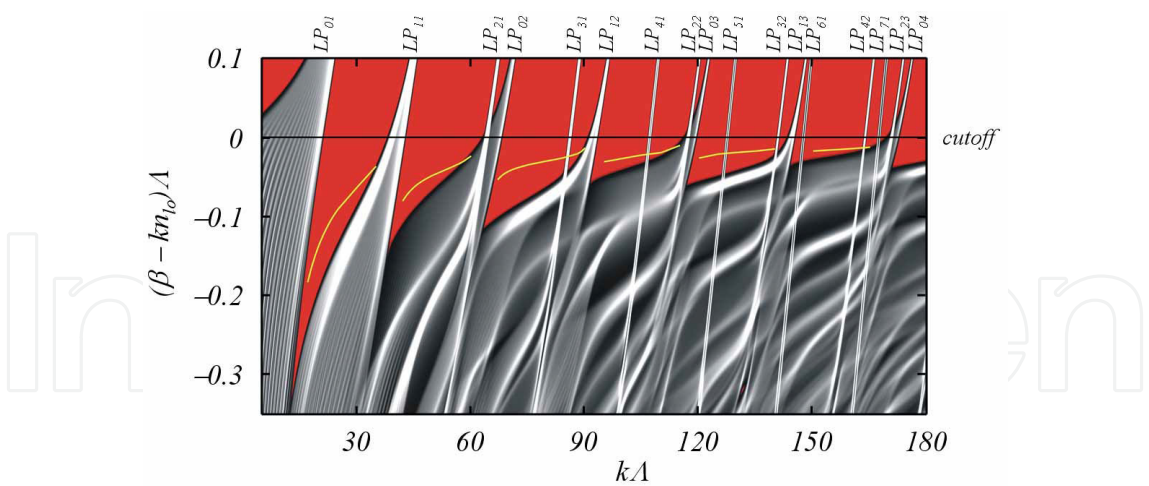
Figure 25. Plots of band structure for an example bandgap fiber. The bandgaps are shown in red. The node modes from which the bands arise are labeled along the top. Density of states (DOS) calculated using the plane-wave method, with light grey corresponding to high DOS. The yellow curve is the "fundamental" core-guided mode [45].
