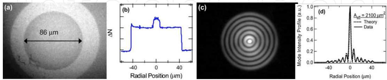
Figure 19. Characteristics of an HOM fiber. The horizontal and vertical scales of the images are identical. (a) Near-field image of a fiber facet, showing the 86μm inner cladding. (b) Refractive-index profile of the HOM fiber, with a core similar to an SMF with an 86μm inner cladding and a down-doped outer trench. (c) Near-field image of the LP_{07} mode at 1600 nm after 12m propagation with a 4.5cm radius bend. (d) Intensity line scan of (c) and theoretical profile: A_{eff} \sim 2100 \mu m^2 [11].
