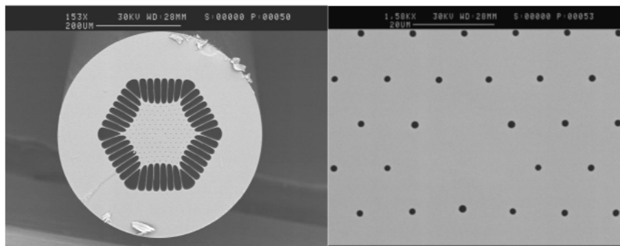
Figure 4. SEM image of the air-clad ytterbium-doped large-mode-area photonic crystal fiber in [26].
