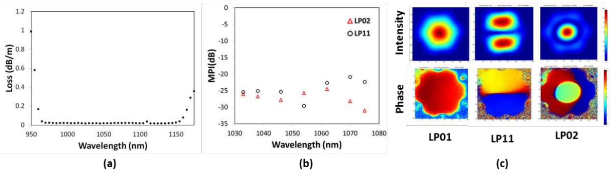
Figure 26. (a) Transmission of the 55μm core all-solid photonic bandgap fiber, (b) measured HOM contents with a S^2 method in a 5m fiber coiled at 70cm diameter, and (c) measured mode images [51].
