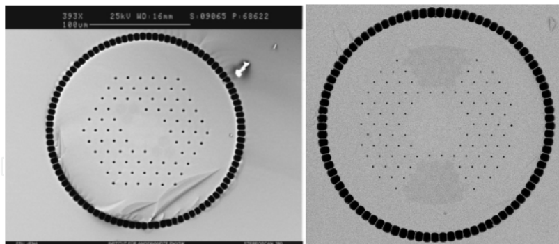
Figure 8. SEM image of the single polarization PCF with an effective area of \sim 700\mu\text{m}^2 [31] (left) and 2300\mu\text{m}^2 (right) [32].
