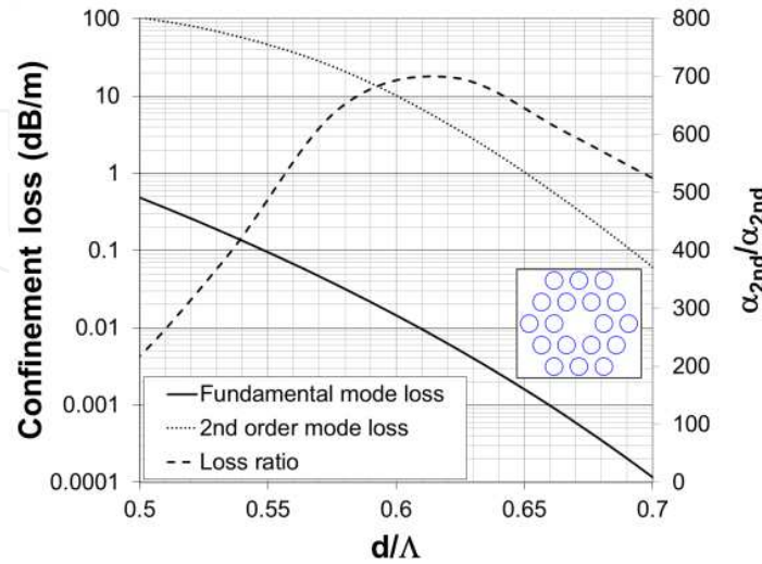
Figure 11. Effect of d/\Lambda on confinement loss and the loss ratio between the second-order mode and fundamental mode for an LCF with two layers of features, \Delta n=1.2 \times 10^{-3} and 2Q=50\mu\text{m} . [35].
