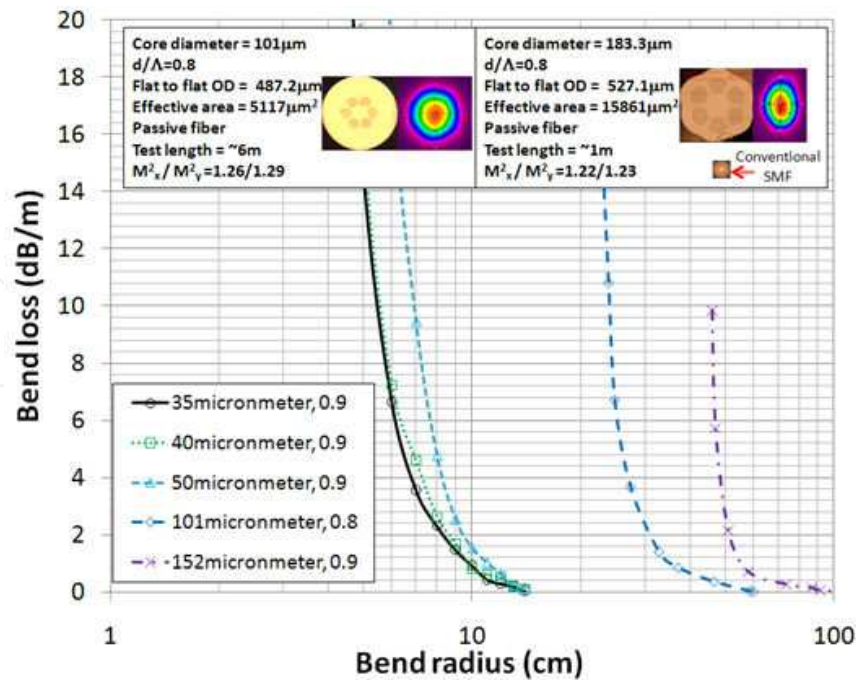
Figure 13. Cross section, measured mode and fiber details are given for the LCF with 101μm core, left inset, and the LCF with 183.3μm core, right inset. Measured bend loss for LCFs with various core diameters [36].
