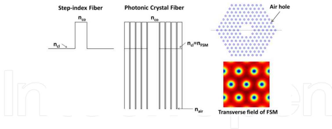
Figure 1. Refractive index of photonic crystal fiber cladding.
