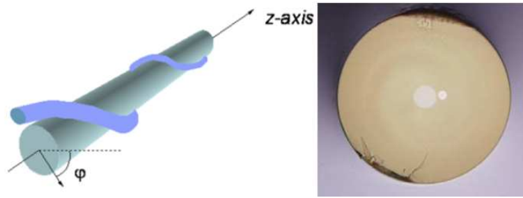
Figure 22. Structure of Chirally-coupled-core fiber [9].
