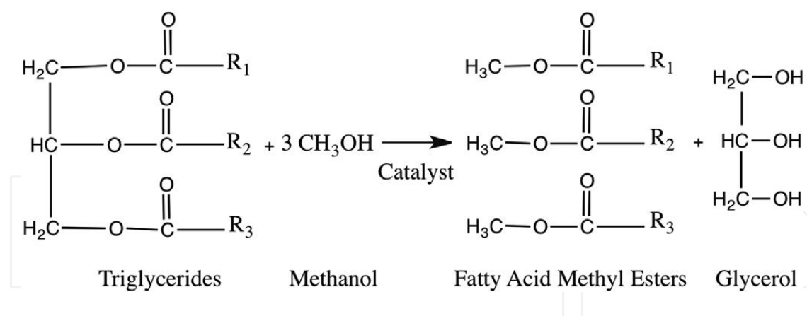
Figure 3. Transesterification reaction to obtain biodiesel.
