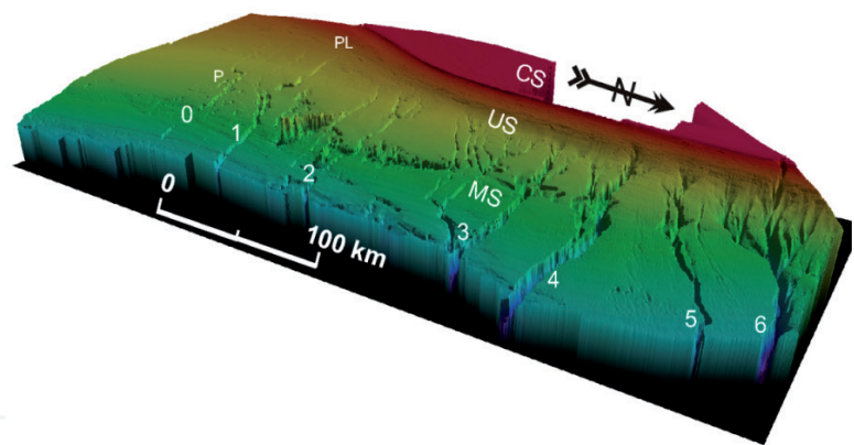
Figure 2. Colour shaded 3D bathymetric map of a segment of the Patagonian Argentinean margin compiled from multi-beam backscatter data. Arabic numbers identify submarine canyons discussed in text. CS=Continental shelf; US=Upper continental slope; MS=Middle continental slope; P=Pockmark; PL=Iceberg plough marks.
