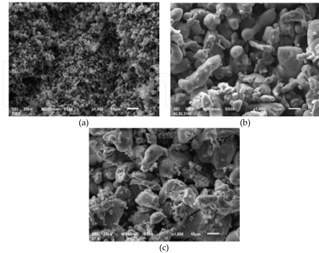
Figure 2. Morphology of powders of: a) titanium diboride, b) AISI 316L austenitic stainless steel and c) mixtures of steel with 8 vol% TiB 2 used in current study.
