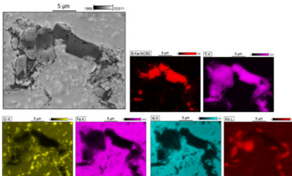
Fig.13 The microstructure of composites with 8 vol% of \text{TiB}_2 (SPS method, sintered at 1100°C, 5 min) with corresponding area analysis (WDS).
