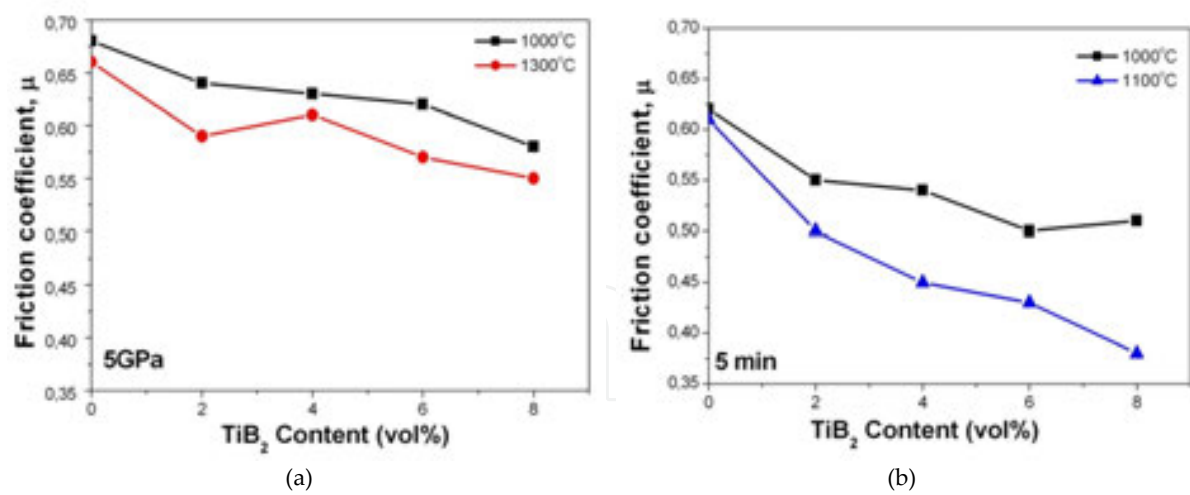
Figure 18. Variation of friction coefficient with \text{TiB}_2 content for composites sintered by: a) HP-HT [54] and b) SPS [53] method.
