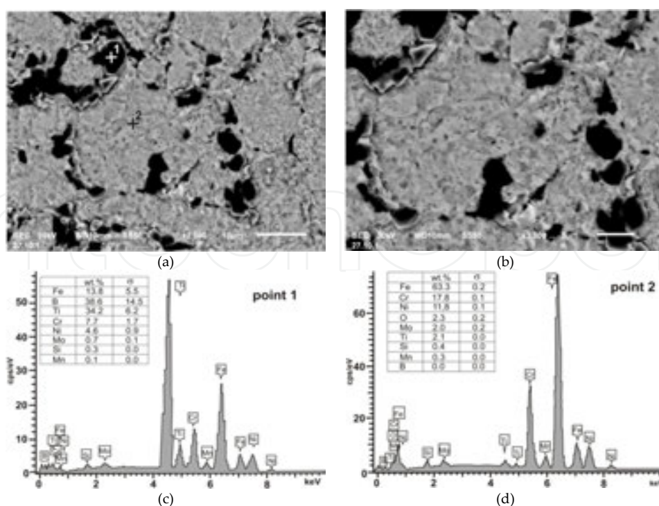
Figure 10. (a, b) The microstructure of composites with 8 vol% of \text{TiB}_2 (HP-HT method, sintered at 1300^\circ\text{C} , 5 GPa) and (c, d) corresponding point analysis (EDS).
