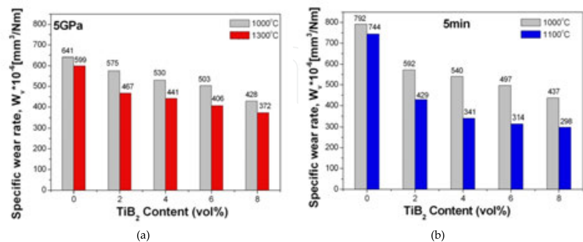
Figure 19. Variation of specific wear rate with \text{TiB}_2 content for composites obtained by: a) HP-HT [54] and b) SPS [53] method.
