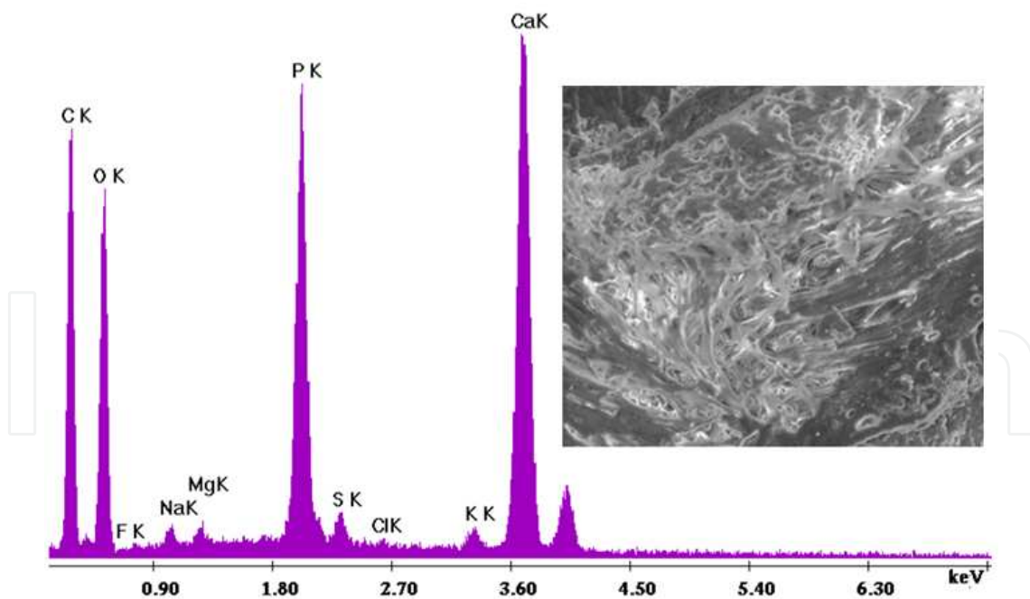
Figure 7. SEM imaging of control enamel, region rich in rod-like microorganisms (scale 300 μm) and their EDAX analysis of the area.
