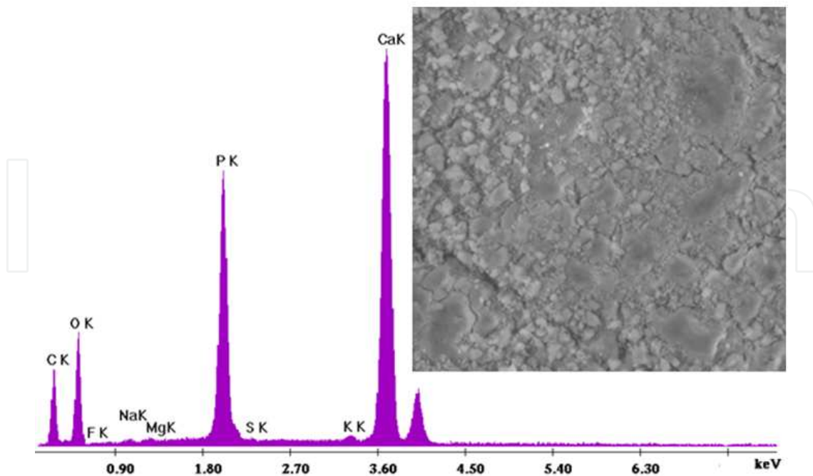
Figure 6. SEM imaging of DS enamel, region rich in mineral deposits (scale 300 μm) and their EDAX analysis of the area.
