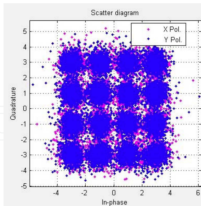
Figure 10. The QAM 16 modulated signal constellation for the transmission distance of 1300 km, BER=10^{-1.83} , CP 1% Conventional CO-OFDM system.
