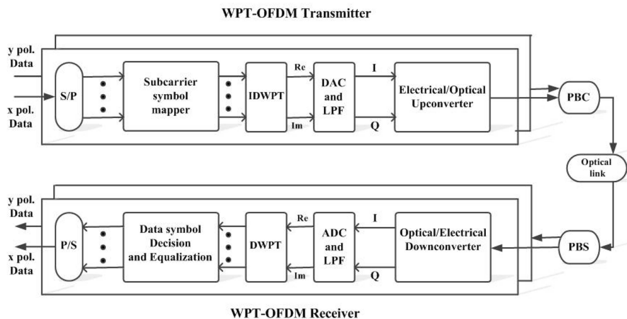
Figure 2. Block diagram of WPT-OFDM communication system. PBC/PBS: polarization beam Combiner/Splitter.
