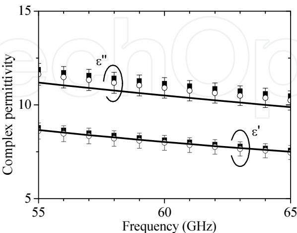
Figure 3. Comparison of our experimental result for the wrist skin permittivity (—) with Gabriel et al. (dry skin) (■) and Alekseev et al. (O) models. Error bars represent \pm 5\% deviations around Gabriel's reference values.
