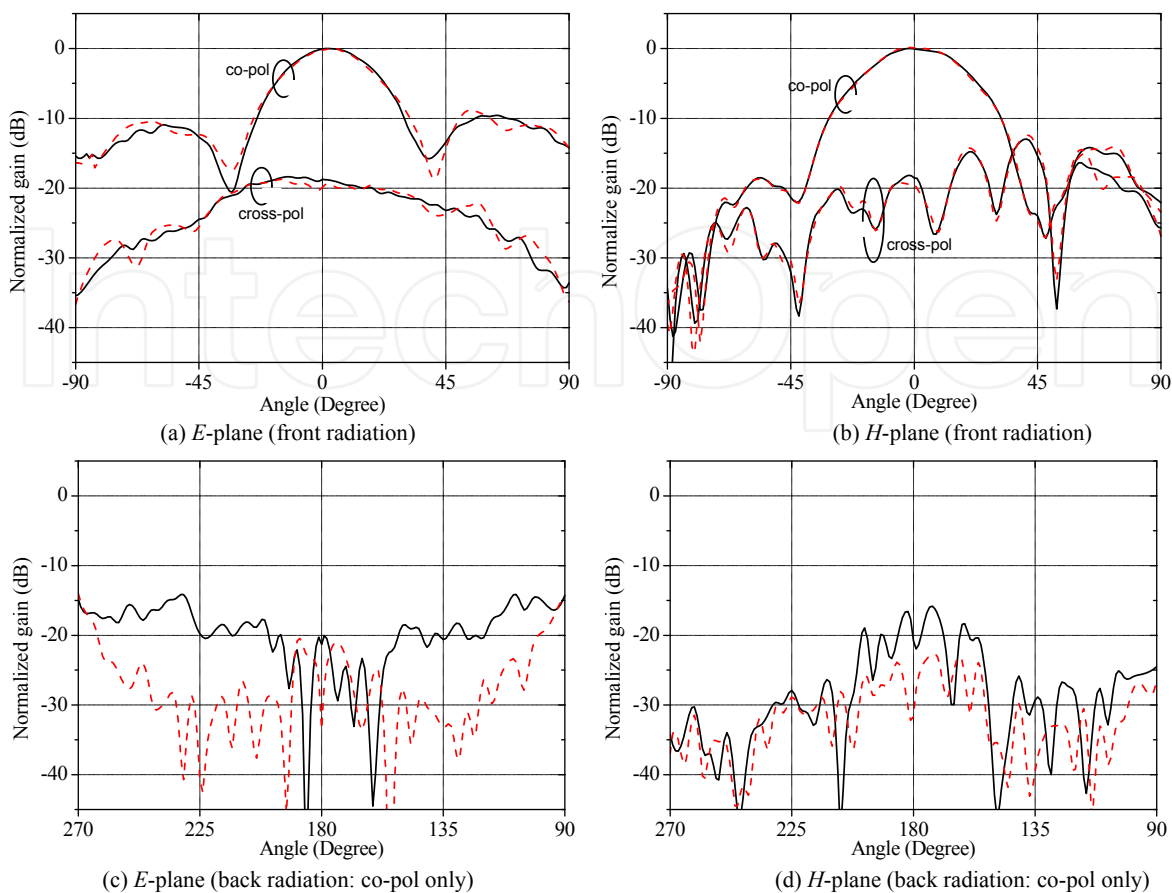
Fig.15. Measured normalized radiation patterns at 60 GHz in E - and H -planes. — Measurement in free space. - - - Measurement on the phantom. Figure 15. Measured normalized radiation patterns at 60 GHz in E - and H -planes. — Measurement in free space. - - - Measurement on the phantom.
