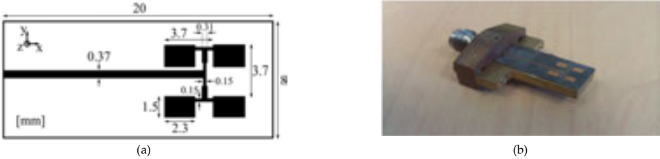
Figure 13. Patch single-layer antenna array at 60 GHz [24]. (a) Schematic representation of the antenna model and dimensions. (b) Manufactured antenna with a V-conductor.
