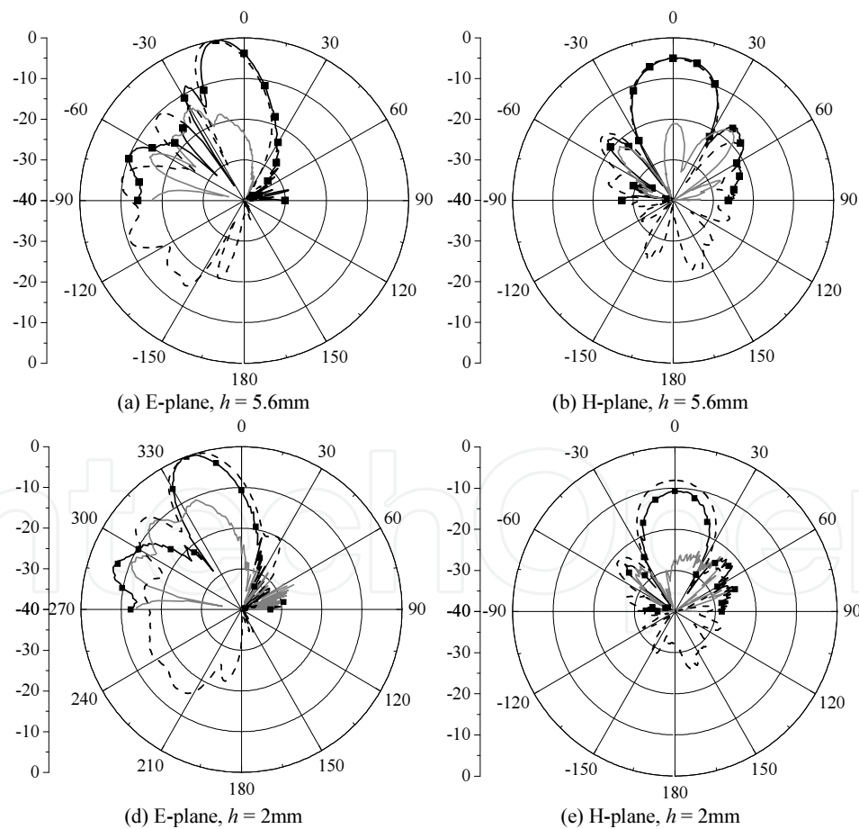
Figure 35. Measured and simulated radiation patterns on the skin-equivalent phantom at 60 GHz. —■— Measured co-pol. — Computed co-pol. — Measured cross-pol. — Computed cross-pol.
