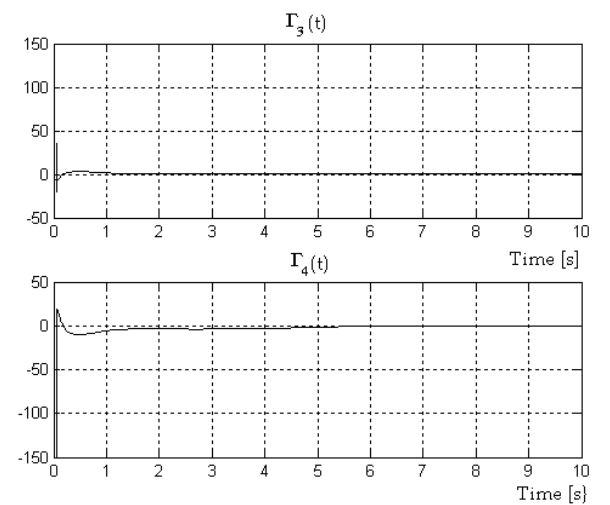
Fig. 13. Stabilization of the five-link biped in vertical posture, torques in the inter-link joints 3 and 4.
