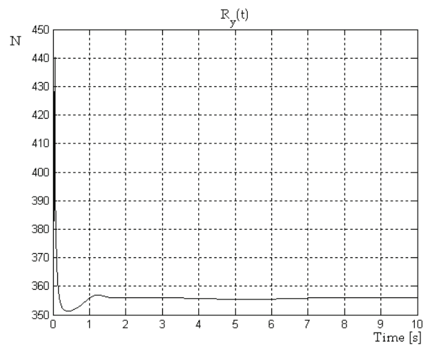
Fig. 14. Stabilization of the five-link biped in vertical posture, vertical component of the ground reaction in the stance leg tip.
