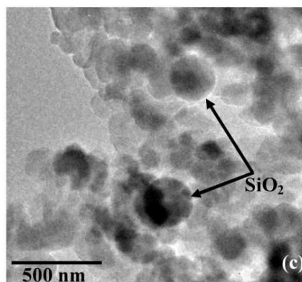
Figure 18. (a) FESEM micrograph of chitosan/polypyrrole/SiO 2 composite. TEM micrographs of (b) Chitosan/polypyrrole/SiO 2 and (c) polypyrrole/SiO 2 composites. (Communicated to Progress in Organic Coatings, Ref. 110, Elsevier)
