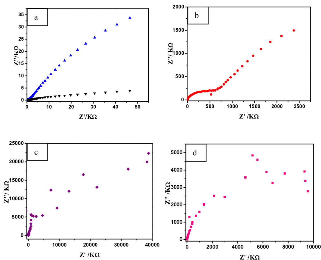
Figure 10. Nyquist plots of epoxy coated (▼) and epoxy with 1.0 wt% (▲), 2.0 wt% (●), 3.0 wt% (◆) and 4.0 wt% (■) loading of polypyrrole/SiO 2 composite (PCs) coated mild steel specimens in 3.5% NaCl solution at room temperature (25±3°C). (Progress in Organic Coatings DOI: 10.1016/j.porgcoat.2014.04.013).
