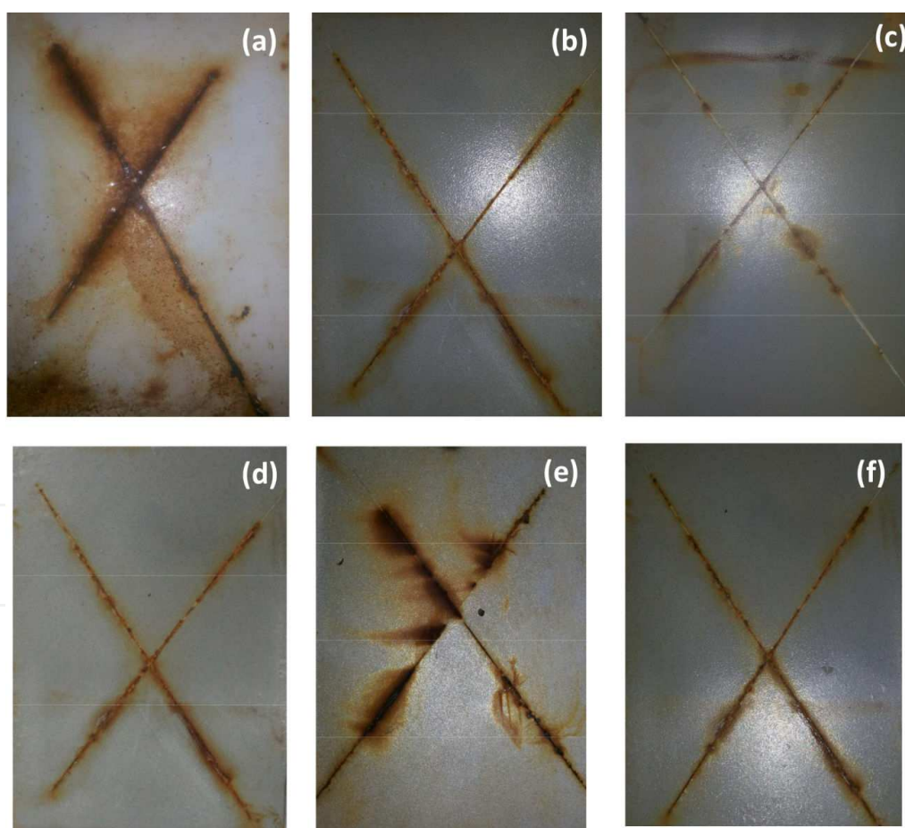
Figure 22. Photographs of (a) epoxy coated and epoxy with (b) 1.0 wt%, (c) 2.0 wt%, (d) 3.0 wt% loading of chitosan/polypyrrole/SiO 2 , (e) chitosan/polypyrrole and (f) polypyrrole/SiO 2 composite coated mild steel specimens exposed to salt spray fog after 65 days. (Communicated to Progress in Organic Coatings, Ref. 110, Elsevier)
