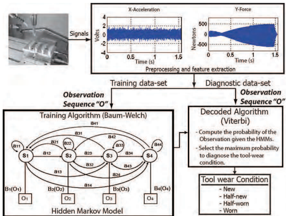
Fig. 13. Flow diagram for monitoring and diagnosis the cutting tool wear condition with continuous HMM. The features from signals are separated into 2 branches. The training branch leads leads to HMM , and the diagnose branch uses the new observations and HMMs to recognize the cutting tool condition.
