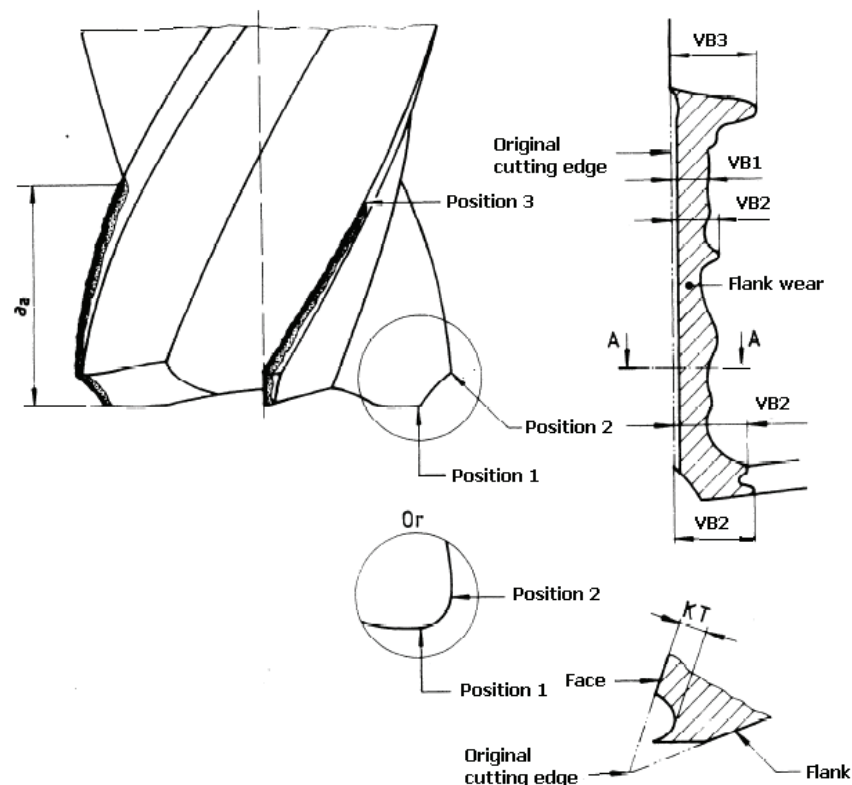
Fig. 3. Different terms in the flank wear are depicted for an end milling cutter (Taken from ISO 8088-2, 1989).
