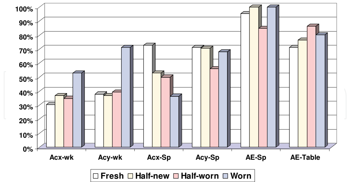
Fig. 15. Performance of the HMM for the different process signals. The results correspond to the obtained success for the testing dataset. A classical test in a diagnosis system is to identify two alarms due to a false classification of cutting tool condition. These alarms are: False Alarm Rate ( FAR ), and False Fault Rate ( FFR ).
