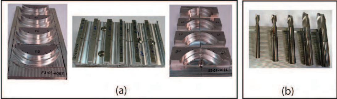
Fig. 2. a) Aluminium workpieces and geometries. b) Cutting tools for the experimentation.
