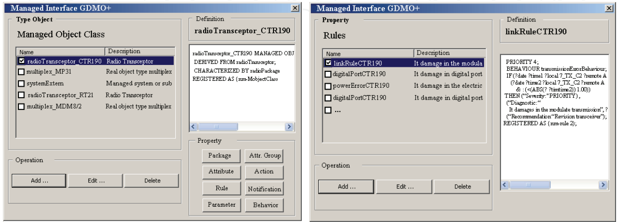
Fig. 13a System Object Classes Dialog Box Fig. 13b System Object Classes Update
