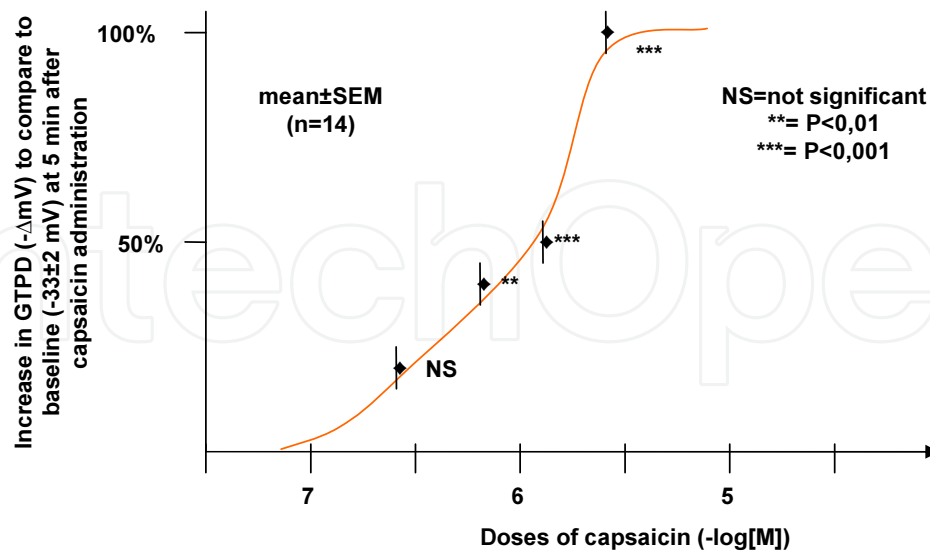
Figure 9. Dose-response curve of capsaicin on the gastric transmembrane potential difference (GTPD) in healthy human subjects (Mózsik Gy. et al., 2005), when the different doses were directly intragastrically via endoscopic channel. The GTPD measurements were carried out at 1, 2, 3, 4, and 5 minutes. The results are expressed at 5 min after capsaicin intragastric application.
