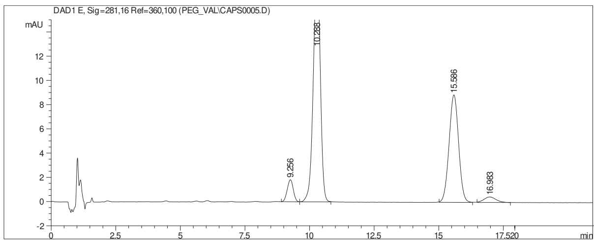
Figure 3. High Pressure Liquid Chromatography (HPLC-DAD) chromatogram of a Natural Capsaicin sample. (Retention times: Capsaicin t_R=10.29 min, Dihydrocapsaicin t_R=15.59 min. Identification of the components was performed by means of the respective USP standards.) (Kuzma M. et al., unpublished results)
