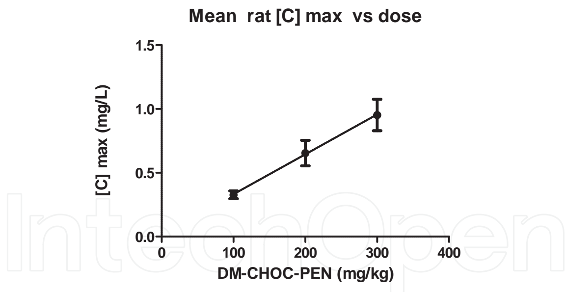
Figure 8. [C]_{\max} vs. dose for 1
