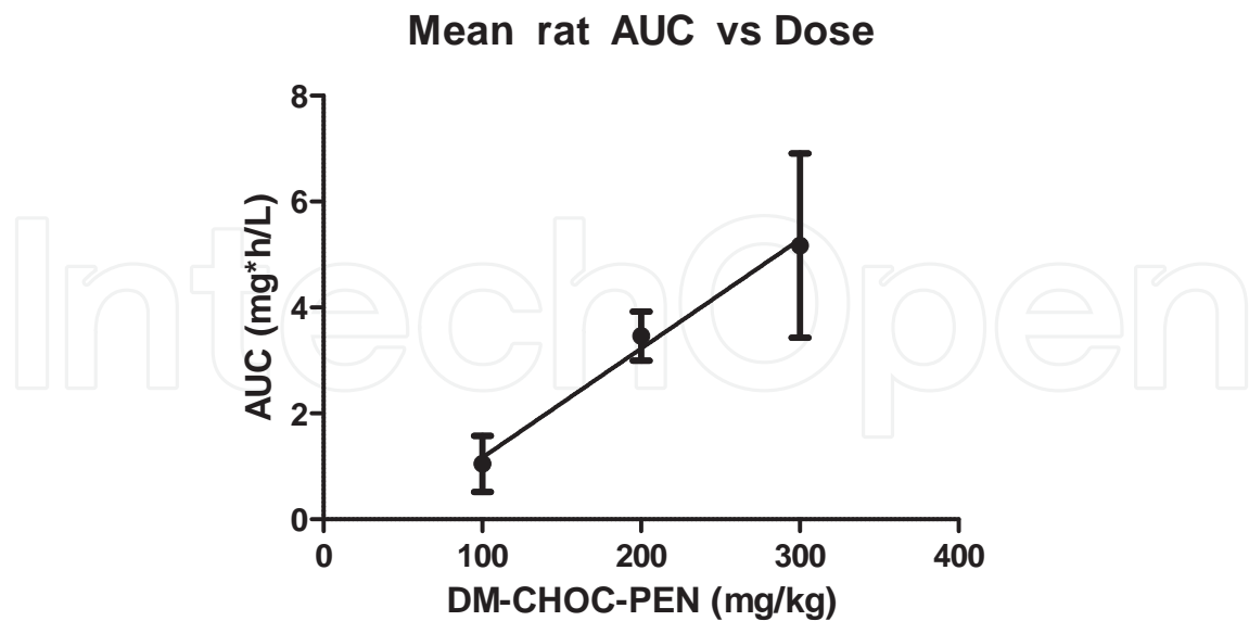
Figure 7. AUC vs. dose for 1
