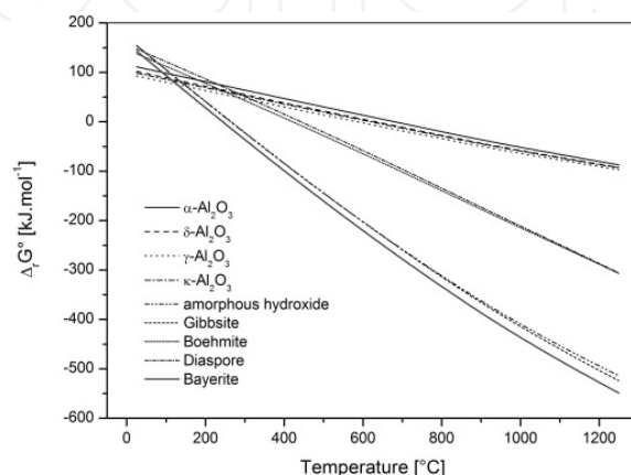
Figure 7. Temperature dependence of \Delta_r G^\circ for the formation of structure unit of \text{SrAl}_2\text{O}_4 from different sources of alumina.
