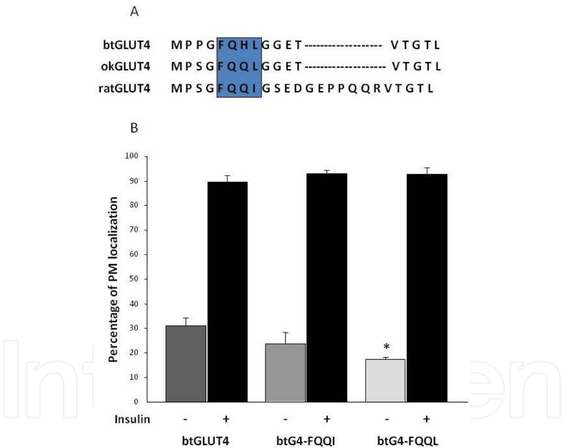
Figure 8. The elevated basal cell surface levels of btGLUT4 are reduced by mutating the F 5 QHL 8 motif. (A) Amino acid sequence alignment of the N-terminal region of rat, brown trout (btGLUT4, AF247395) and coho salmon (okGLUT4, AF502957) GLUT4 molecules. The box encloses the important trafficking motif F 5 QQI 8 partially conserved in the fish species. (B) Differentiated 3T3-L1 adipocytes expressing either btGLUT4 or any of the two point mutants (btGLUT4-FQQI or btGLUT4-FQQL) were incubated with or without insulin (100 nM, 30 min). Data is presented as percentage (mean ± SEM) of cells showing a complete plasma membrane (PM) rim obtained by counting 100 cells per condition in 3 independent experiments. Statistical analysis was performed by unpaired t-test against the wild type btGLUT4 at basal or insulin-stimulated conditions respectively (* denotes significance at p < 0.05).
