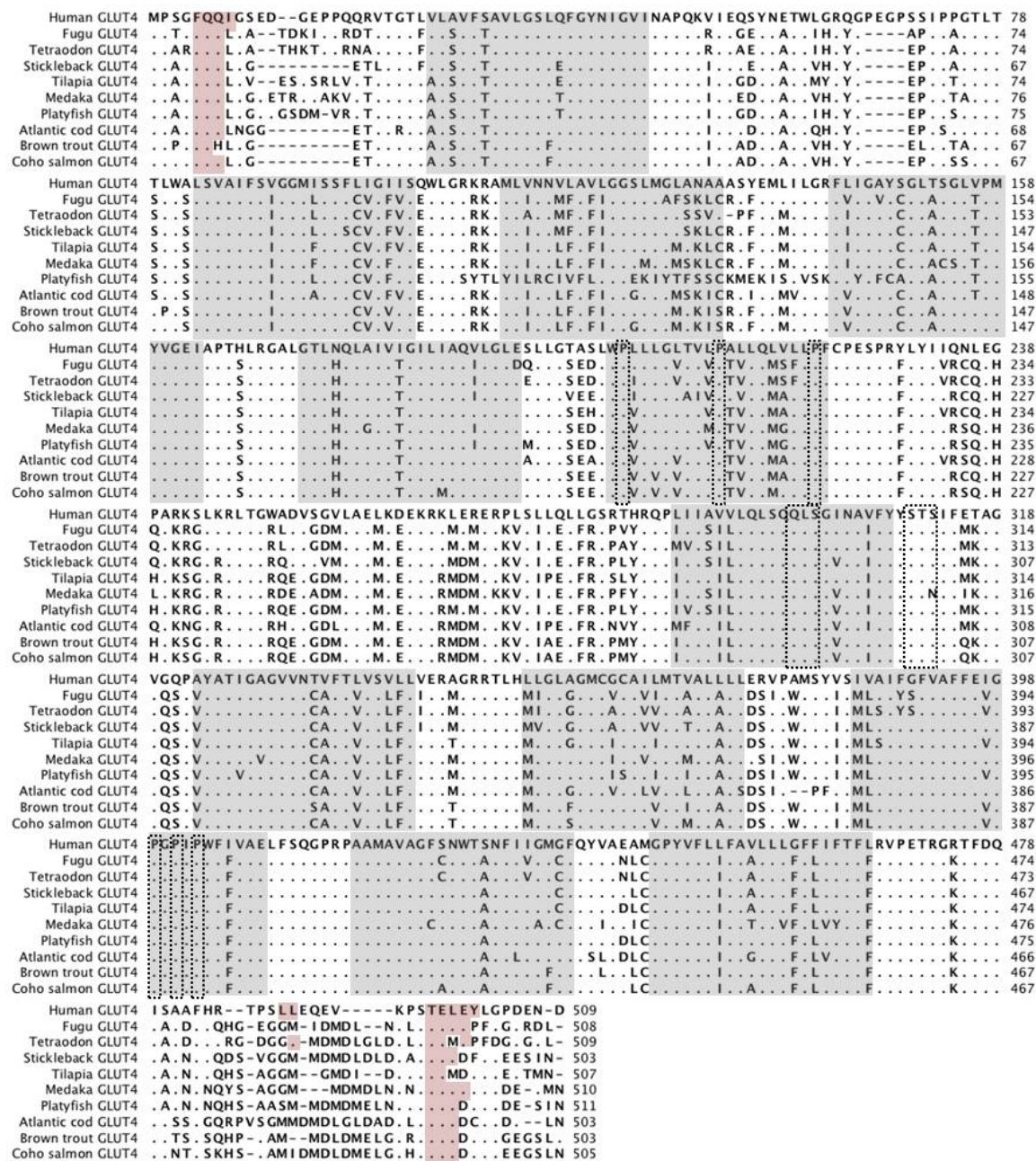
Figure 6. Multiple alignment of GLUT4 protein sequences. Identical residues identified using ClustalW are indicated as dots. Grey boxes: Transmembrane domains. Red boxes: Important motifs for GLUT4 trafficking. Dashed box: Important motif for glucose transport. Gene IDs and accession numbers were retrieved from public databases-Human: ENSG00000181856; Fugu: ENSTRUG00000011935; Tetraodon: ENSTNIG00000010138; Tilapia: ENSO-NIG00000018958; Stickleback: ENSGACG00000019384; Medaka: ENSORLG00000006341; Platyfish: ENSX-MAG00000015723; Atlantic cod: AAZ15731.1; Brown trout: AAG12191.1; Coho Salmon: AAM22227.1.
