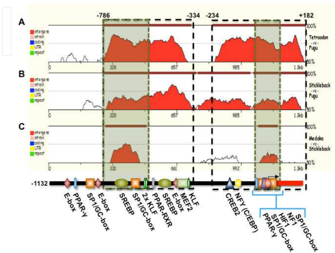
Figure 4. Conservation profile of the promoter region of known fish GLUT4 genes. Sequence elements of significant length ( \geq 100 nucleotides) that show higher than 60% of homology are highlighted in red and depicted with the dark-red rectangles on the top of each graph. The sequence comparison between the Fugu and Tetraodon (A), Fugu and Stickleback (B) and Stickleback and Medaka (C) GLUT4 promoters is shown. The horizontal axis represents the position of the nucleotides within the 1314 bp sequence compared, starting at the 5' end. The vertical axis represents the percent of identity between the aligned genomes. In the bottom, a schematic representation of the -1132 Fugu GLUT4 gene promoter highlighting the most relevant predicted binding sites is shown. The open boxes delineating the regions comprised between -786/-334 and -234/+182 nucleotides represent conserved areas in fish GLUT4 gene promoters. Adapted from [30].
