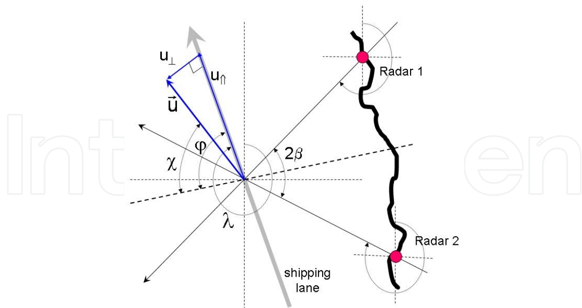
Figure 13. Geometry of bistatic illumination, with current vector and shipping lane
