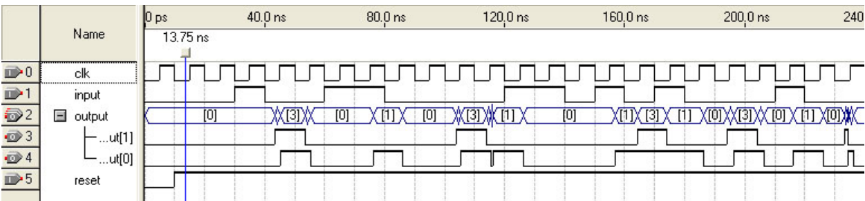
Figure 12. HDB3 line code Simulation in behavioral Verilog.
