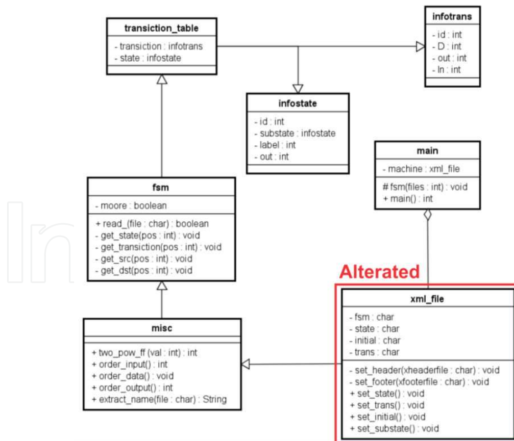
Figure 26. Class diagram of the SF 2 XML tool.
