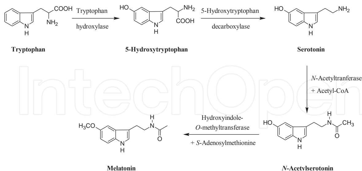
Figure 2. Biosynthetic pathway of melatonin.
