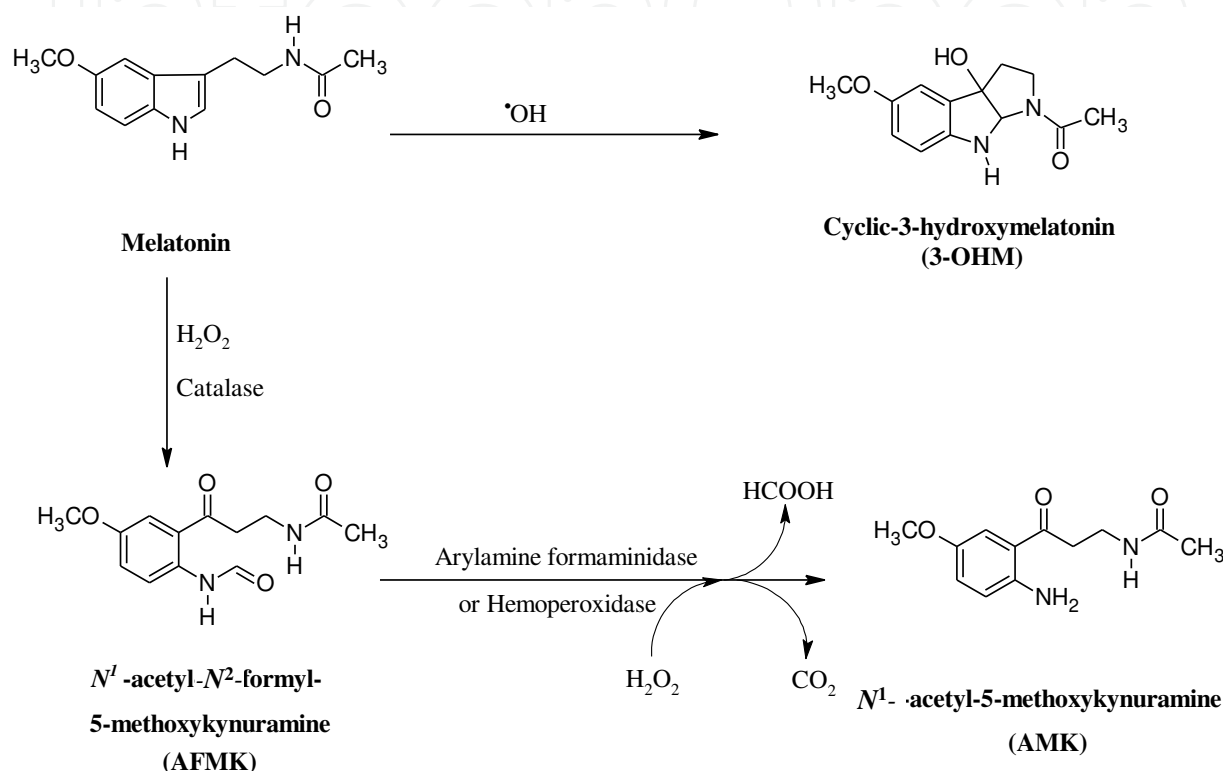
Figure 3. Melatonin oxidation.
