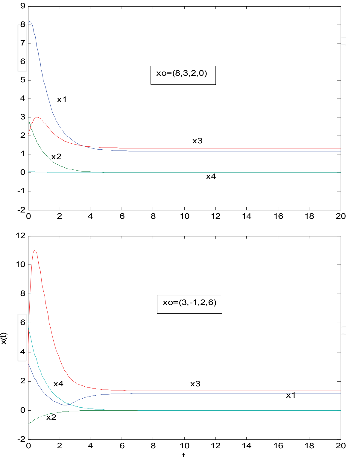
Fig. 5.14. Example 6: The transient behavior of the neural network model, Yashtini and Malek [4] using two different set of the initial points.
