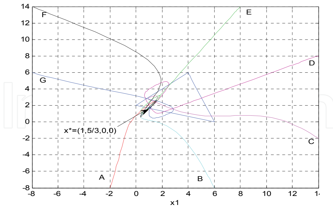
Fig. 5.10. Example 3: The transient behavior of x(t)=(x_1(t),x_2(t)) , using the recurrent neural network model proposed by Yashtini and Malek [4].
