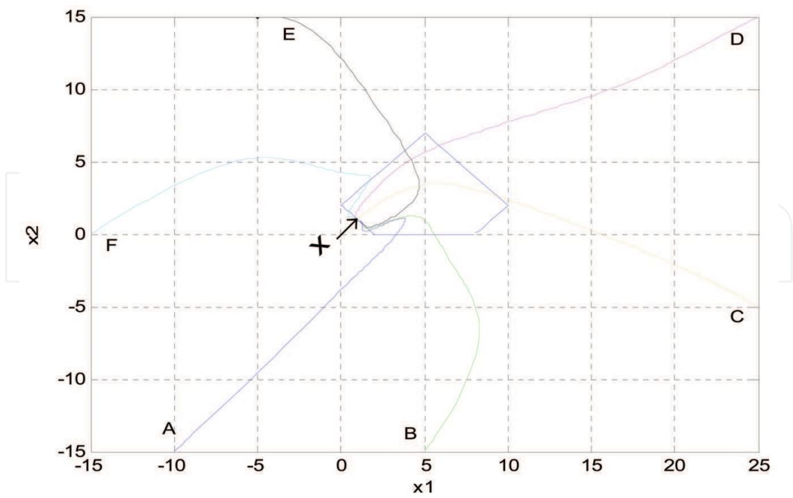
Fig. 5.8. Example 1: trajectories with initial points outside the feasible region using (Model 3).
