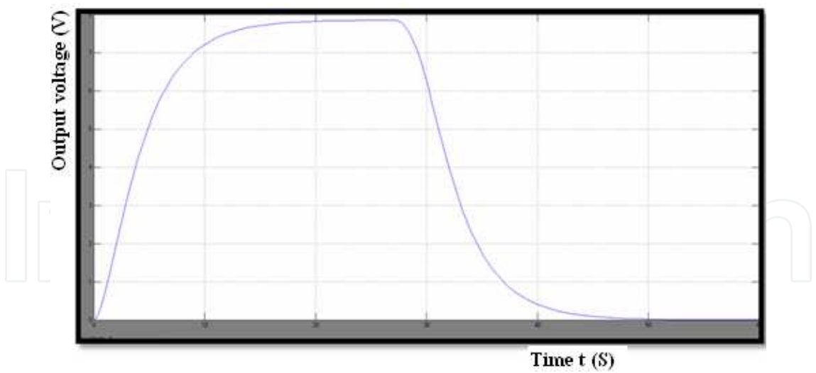
Figure 19. SIMULINK simulation of the train model
