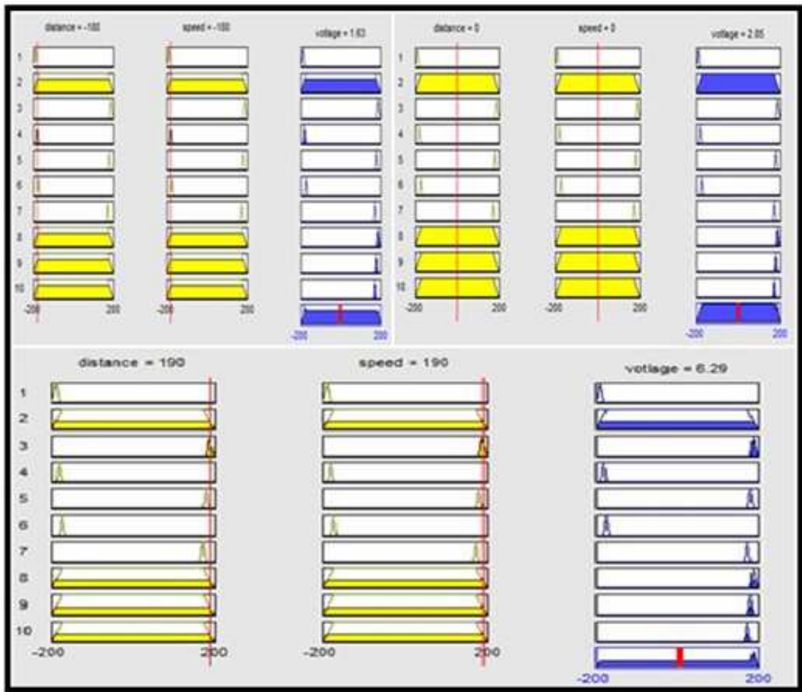
Figure 17. Deffuzification process
