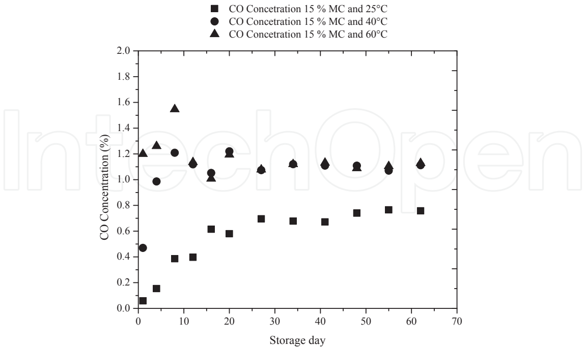
Figure A 5. Concentration of CO for wood pellet with 15% moisture concentration over 62 days at 25°C, 40°C and 60°C
