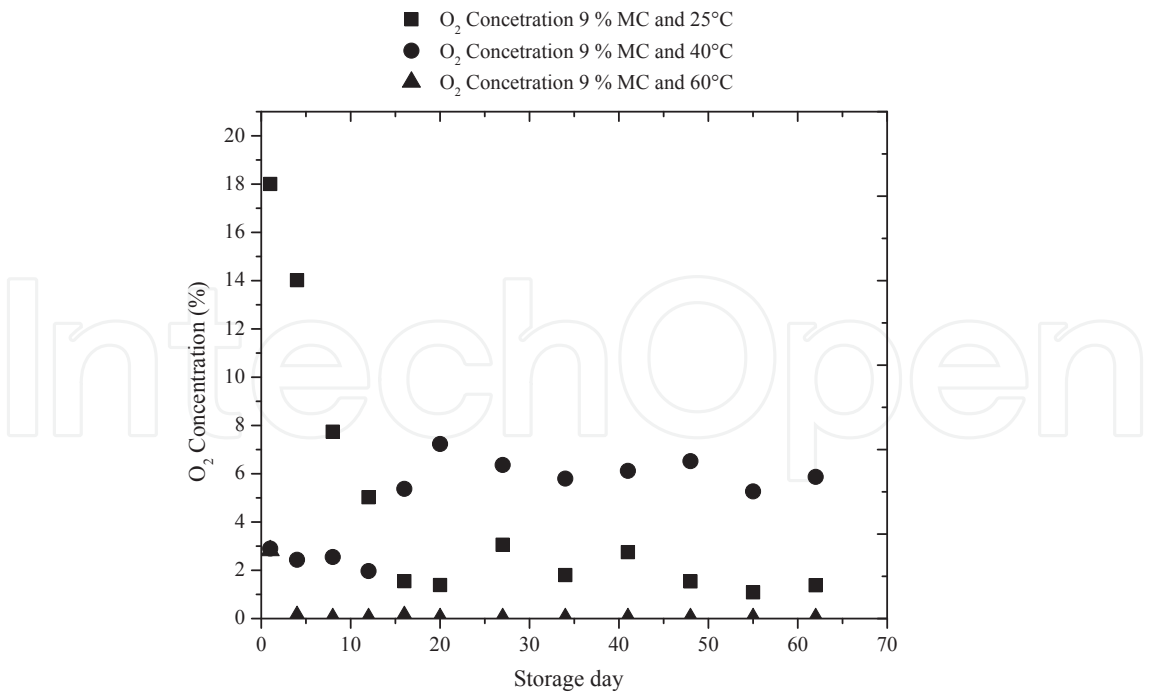
Figure A 10. Oxygen depletion for wood pellet with 9% moisture content over 62 days at 25°C, 40°C and 60°C
