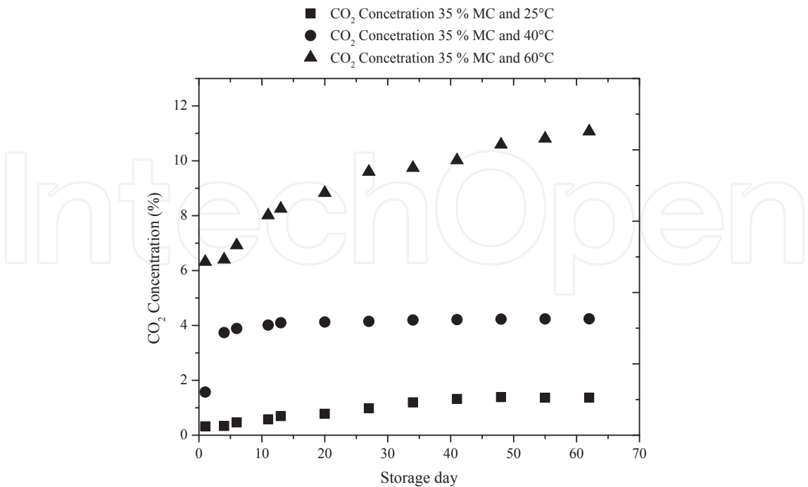
Figure A 3. Concentration of CO 2 for wood pellet with 35% moisture content over 62 days at 25°C, 40°C and 60°C
