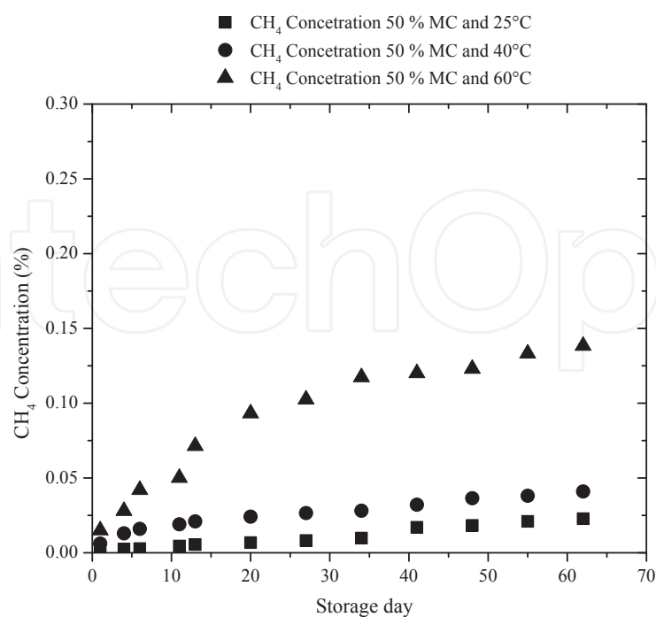
Figure 6. Concentration of \text{CH}_4 for emissions from wood pellet with 50% moisture content over 62 days at 25°C, 40°C and 60°C
