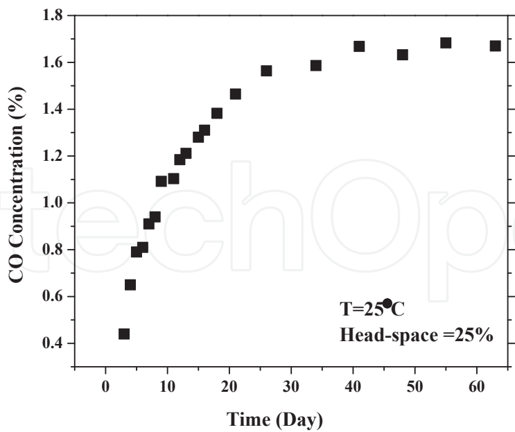
Figure 13. CO concentration in head-space of the silo as a function of storage time for wood pellets. (G0 head-space gas sampling port) [Concentrations are volume percentage]
