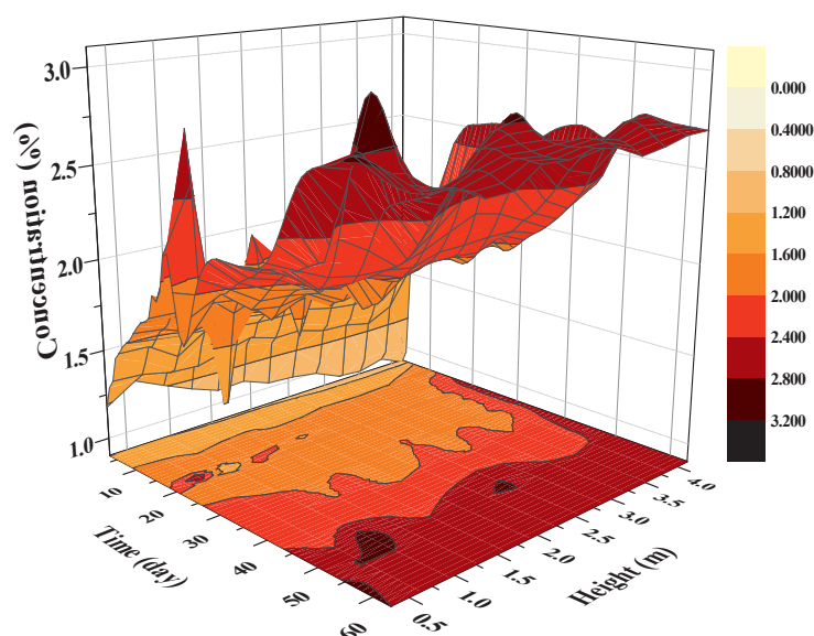
Figure 16. map of \text{CO}_2 concentration in the silo at all locations (G0 to G13) during 63 days of storage [Concentrations are volume percentage]
