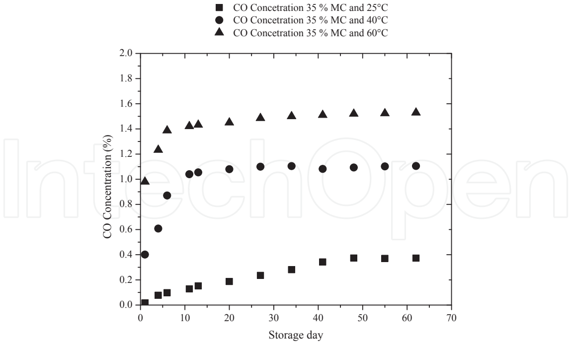
Figure A 6. Concentration of CO for wood pellet with 35% moisture content over 62 days at 25°C, 40°C and 60°C
