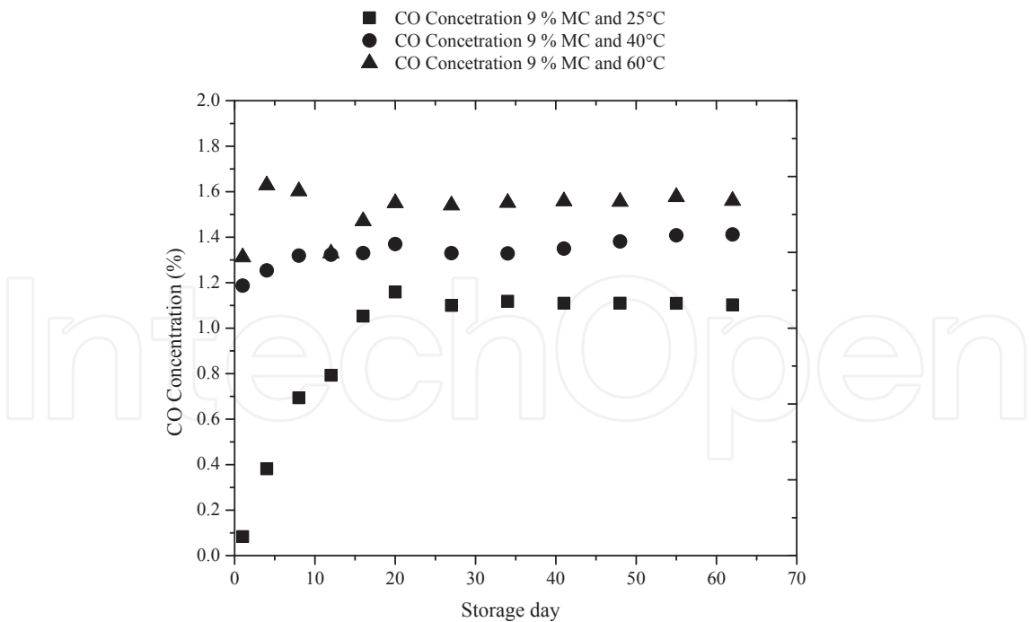
Figure A 4. Concentration of CO for wood pellet with 9% moisture concentration over 62 days at 25°C, 40°C and 60°C
