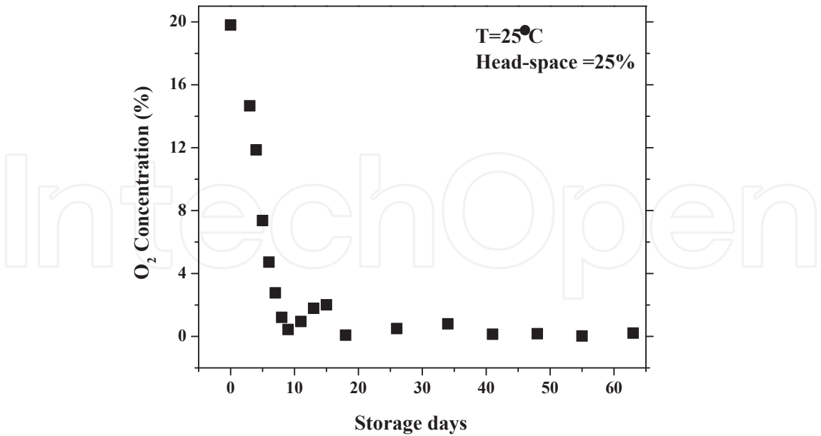
Figure 15. O 2 concentration in head-space of the silo as a function of storage time for wood pellets. (G0 head-space gas sampling port) [Concentrations are volume percentage]
