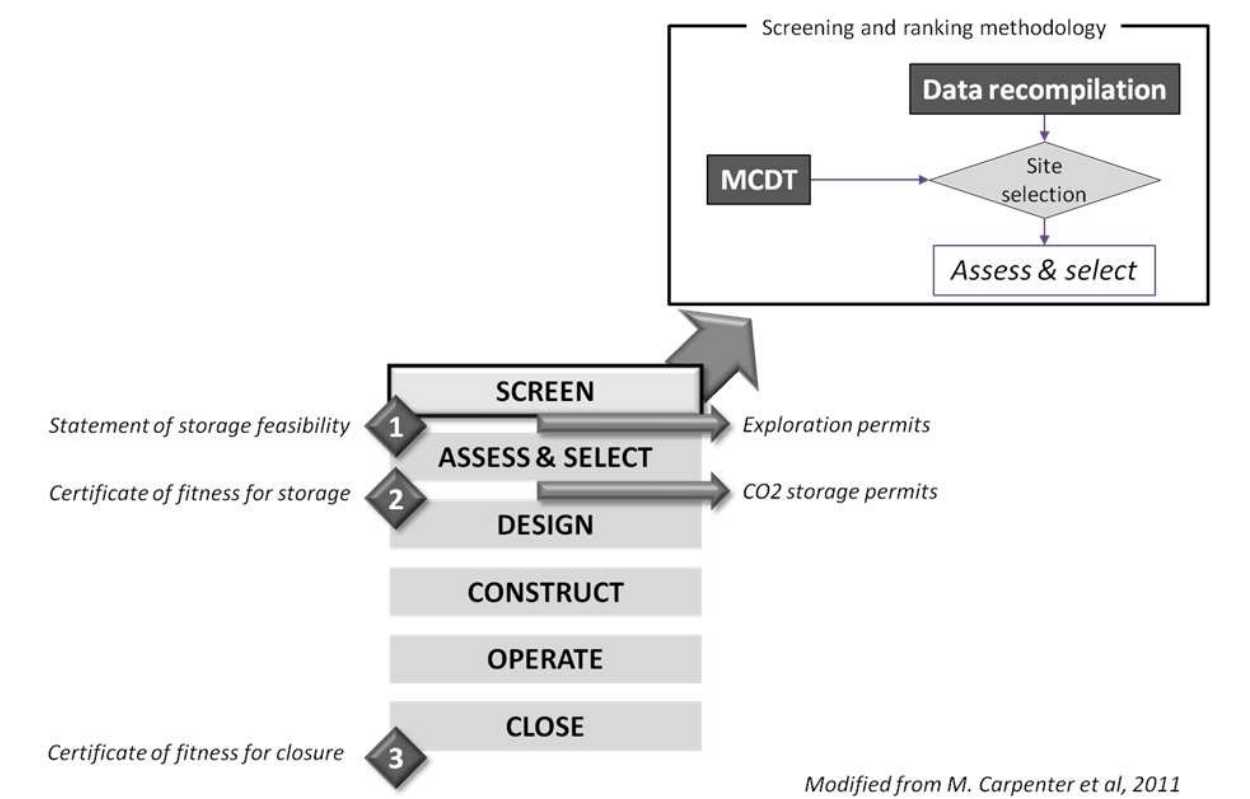
Figure 1. Work flow proposed for basin screening (Definition phase)
