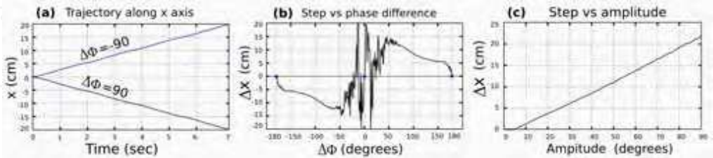
Figure 24. Experiments for the Locomotion in 1D of an 8 module pitch-connecting robot There are some peaks in which it changes abruptly. When the k is equal or greater than two (stability condition) both the trajectory and the pitching angle are smooth. Now there is no instability in the locomotion, as stated by the locomotion principle 3.
