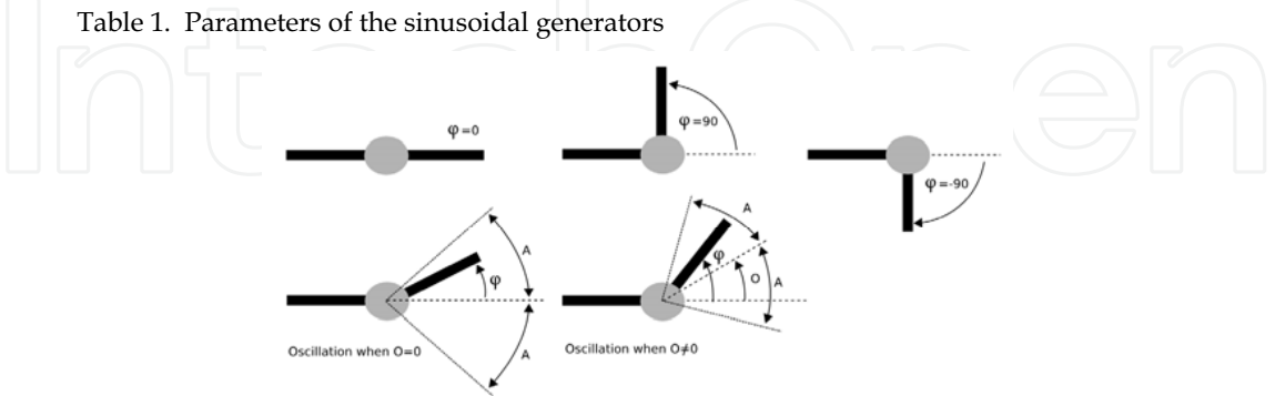
Figure 5. The parameters of the sinusoidal generators
