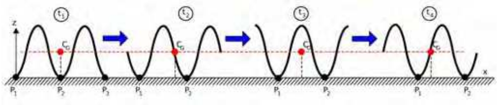
Figure 12. Stability of a pitch-connecting robot when its body wave has the value of two ( k=2 )
