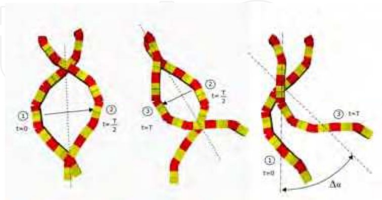
Figure 17. A pitch-yaw connecting robot performing the rotating gait with kh=1
