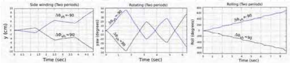
Figure 29. Experimental results for the pitch-yaw-pitch (PYP) minimal configuration
