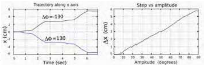
Figure 26. Experiments for the locomotion of the pitch-pitch minimal configuration The simulation results for the minimal pitch-pitch (PP) configuration are shown in Fig. 26. The trajectory along x axis during two periods is shown in the left. The locomotion is not uniform. There are regions where the robot remains stopped and the other regions where the robot can move. When the sign of \Delta\Phi is changed, the movement direction is performed in the opposite. The step also increases with the amplitude, as shown in the right.
