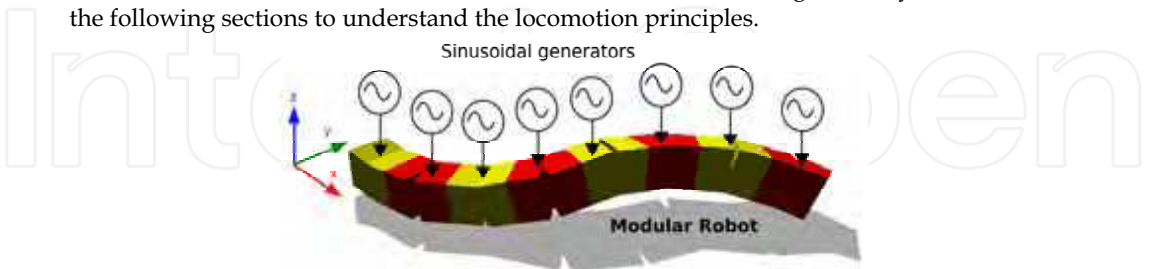
Figure 4. Control approach for the locomotion of pitch and pitch-yaw connecting modular robots
