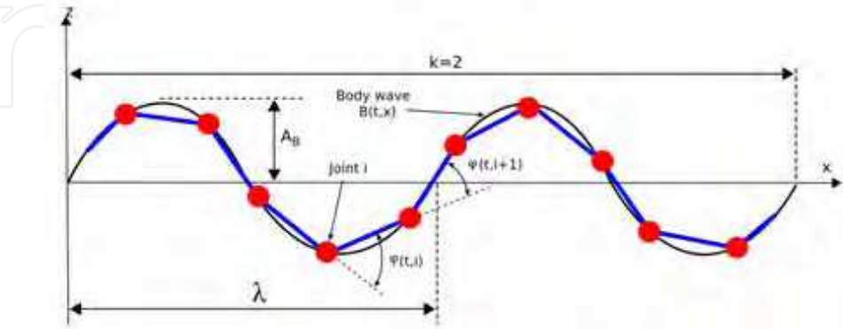
Figure 9. A pitch-connecting modular robot at instant t , the body wave and its parameters
