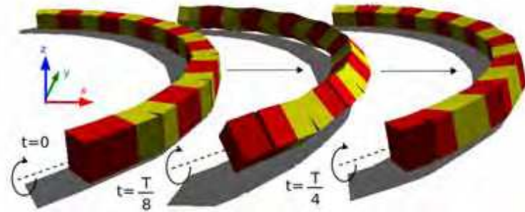
Figure 18. A pitch-yaw connecting robot performing the rolling gait
