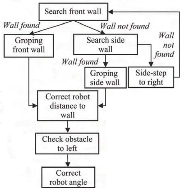
Fig. 5. Groping locomotion algorithm.
