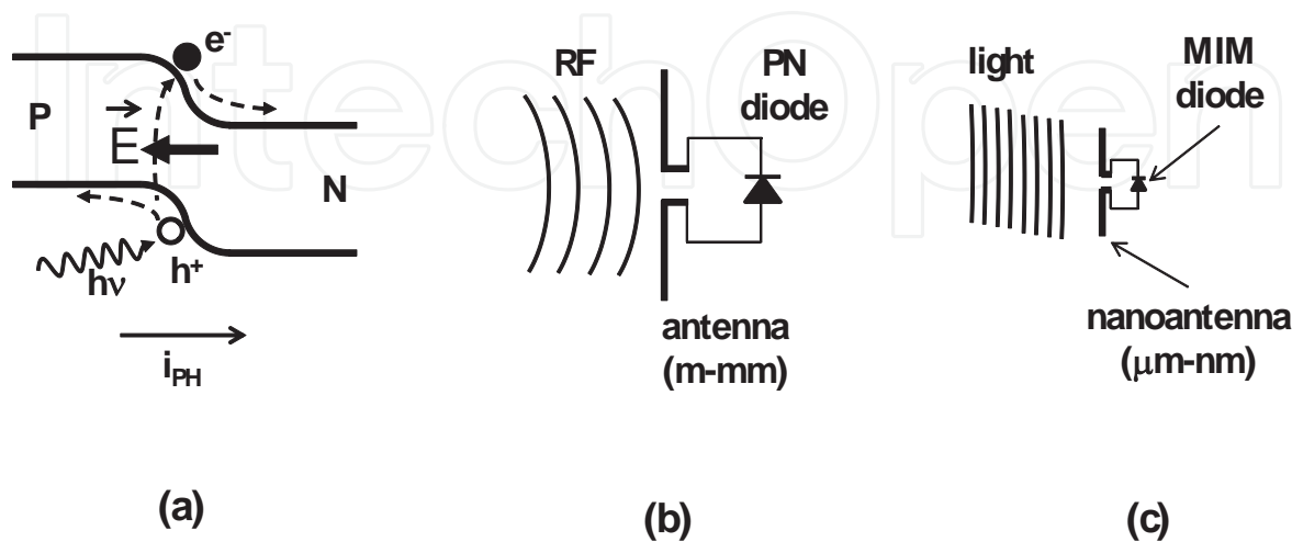
Figure 3. Scheme of the operation principle of three different technologies used to harvest energy from the electromagnetic spectrum. (a) Photovoltaic technology (PV), (b) radiofrequency rectenna technology (RFR) and (c) optical rectenna technology (OR).
