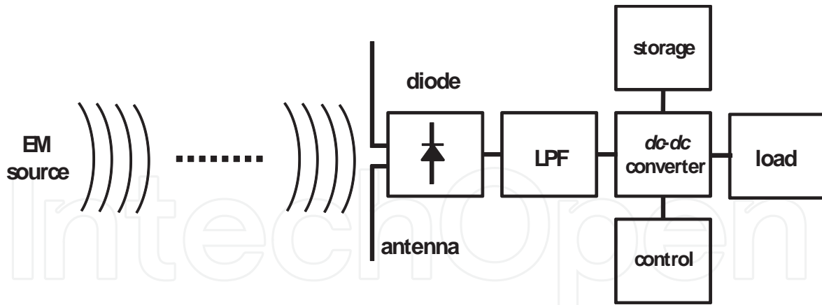
Figure 9. Block diagram of a rectenna.
