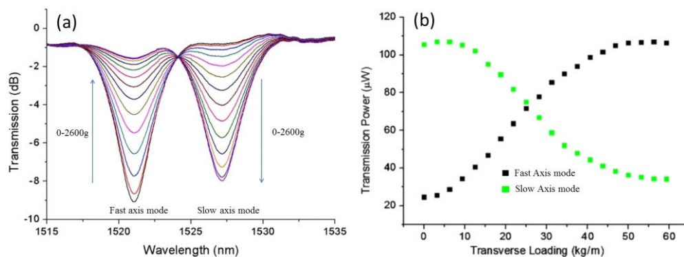
Figure 23. (a) Transmission spectral evolution of the ETFG with transverse load from 0 to 2600g applied on the slow-axis of the ETFG and the support fibre. (b) Power evolution of the ETFG loading sensor using SWL and power meter.
