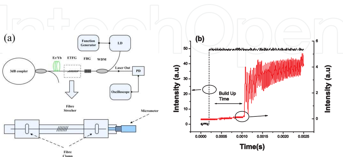
Figure 12. (a) Schematic diagram of the ETFG based fibre laser torsion sensor system; (b) Typical built-up time trace of the fibre laser observed on a digital oscilloscope. Modulation signal is shown in black dotted line; laser output signal is shown in red solid line.
