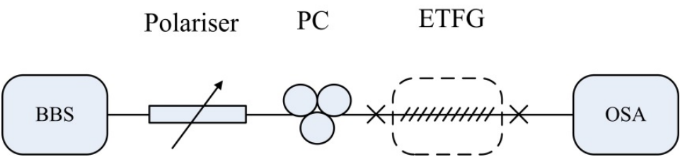
Figure 8. Typical measurement schematic for characterising ETFG.
