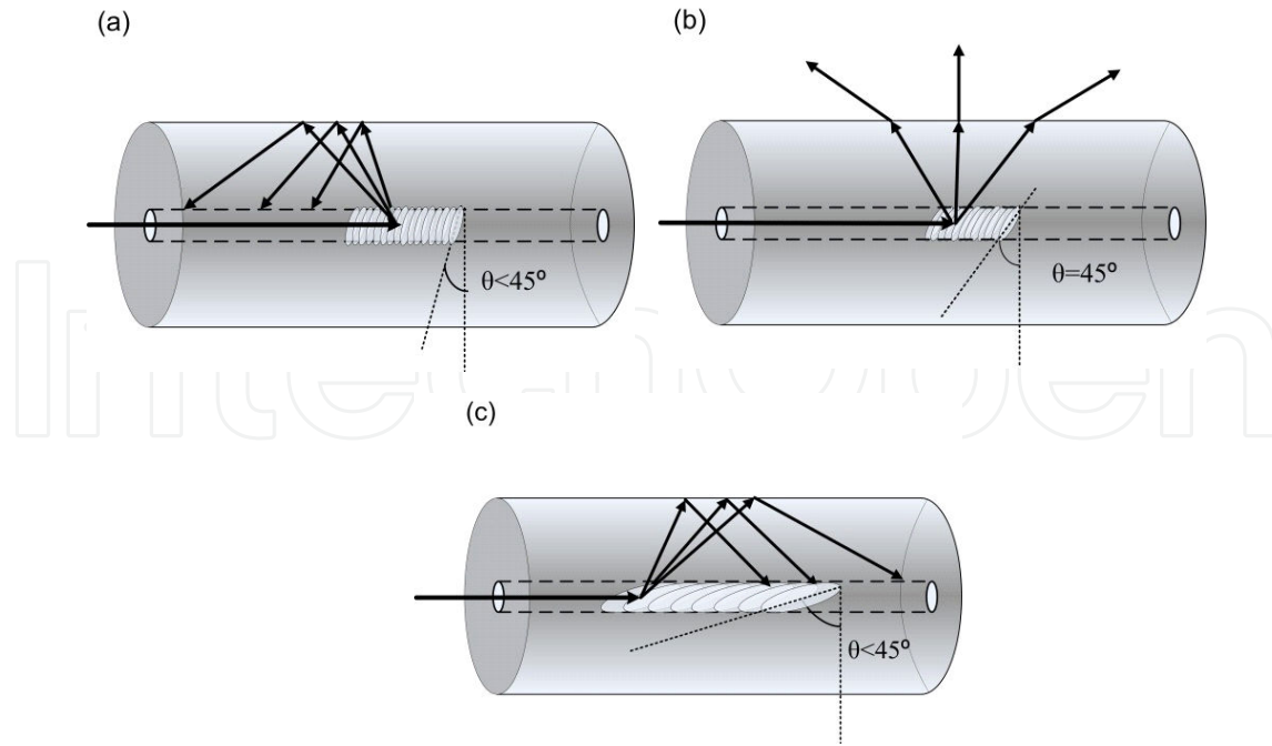
Figure 2. Schematic of light coupling of TFGs with tilted angle (a) < 45^\circ ; (b) = 45^\circ ; (c) > 45^\circ .
