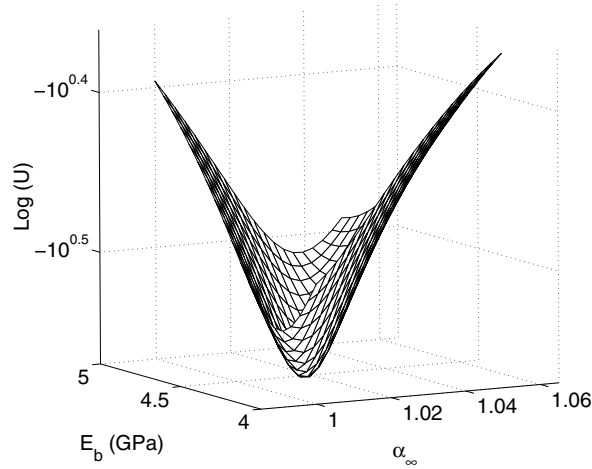
Figure 17. Variation of the minimization function U with the the Young modulus of the skeletal frame E_b and the tortuosity \alpha_\infty .
