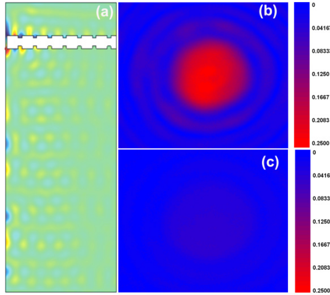
Figure 6. (a) Calculated far-field pressure amplitude distribution at 0.71 MHz in the axial symmetry coordinates. (b) Experimentally scanned far-field (~15 wavelengths from the transmission side of the plate surface) pressure magnitude distributions in an area of 40x40 mm 2 , for the bull’s eye structure at 0.71 MHz. (c) Same as (b), for the reference sample. Reprinted with permission from Appl. Phys. Lett. 92, 124106 (2008). Copyright 2008 American Institute of Physics.
