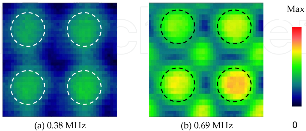
Figure 8. The measured distribution of pressure field at the rear surface of the hole array a=2.0 , r=0.6 , and t=1.6 mm for two resonance frequencies 0.38MHz ( a/\lambda=0.51 ) and 0.69MHz ( a/\lambda=0.93 ). The holes are delineated by dashed lines.
