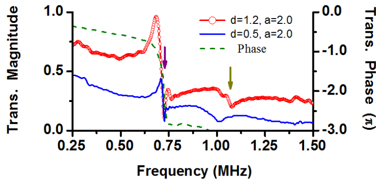
Figure 2. Acoustic transmissions at normal incidence through the hole arrays with the same lattice constant, 2.0 mm, and the same thickness, 0.5 mm, but different diameters as denoted. The measured transmission phase curve is for the hole array: d = 1.2 , a = 2.0 , and t = 0.5 mm. The arrows indicate the Wood's anomalies, \lambda = a and \lambda = a / \sqrt{2} . Reprinted with permission from J. Appl. Phys. 104, 014909 (2008). Copyright 2008 American Institute of Physics.
