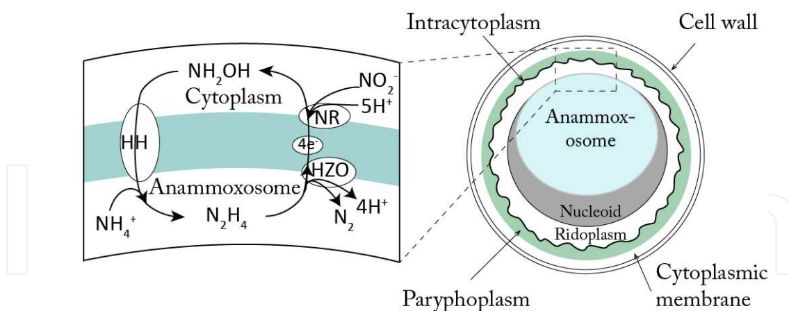
Figure 3. Morphology of the anammox cell and proposed model for the anammox process. HH, hydrazine ( \text{N}_2\text{H}_4 ) hydrolase; HZO, hydrazine oxidizing enzyme; NR, nitrite reducing enzyme [160].
