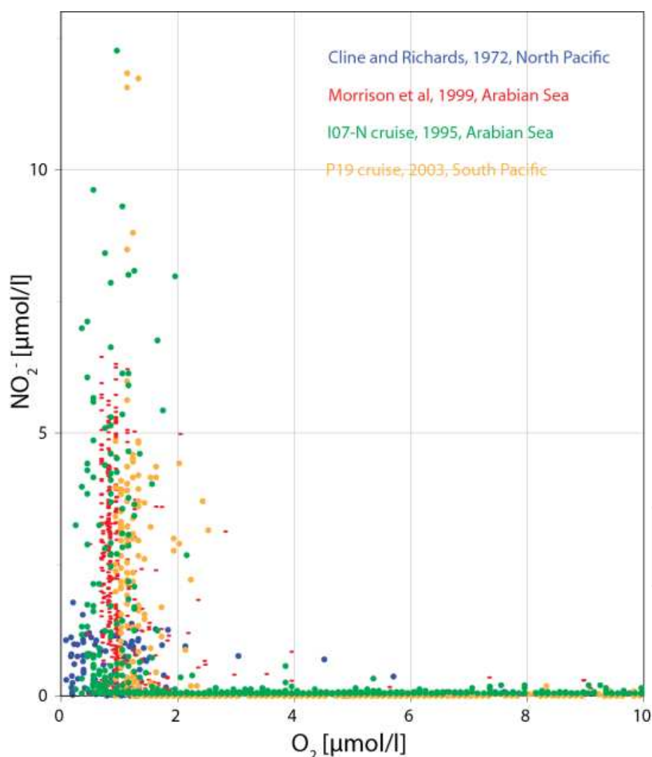
Figure 4. Dissolved oxygen versus nitrite for OMZs. Presented data are taken from publically available cruises I07-N, P19 ( http://woce.nodc.noaa.gov/woce_v3/wocedata_2/bathymetry/default.htm ) and publications of Cline & Richards [182] and Morisson [183].
