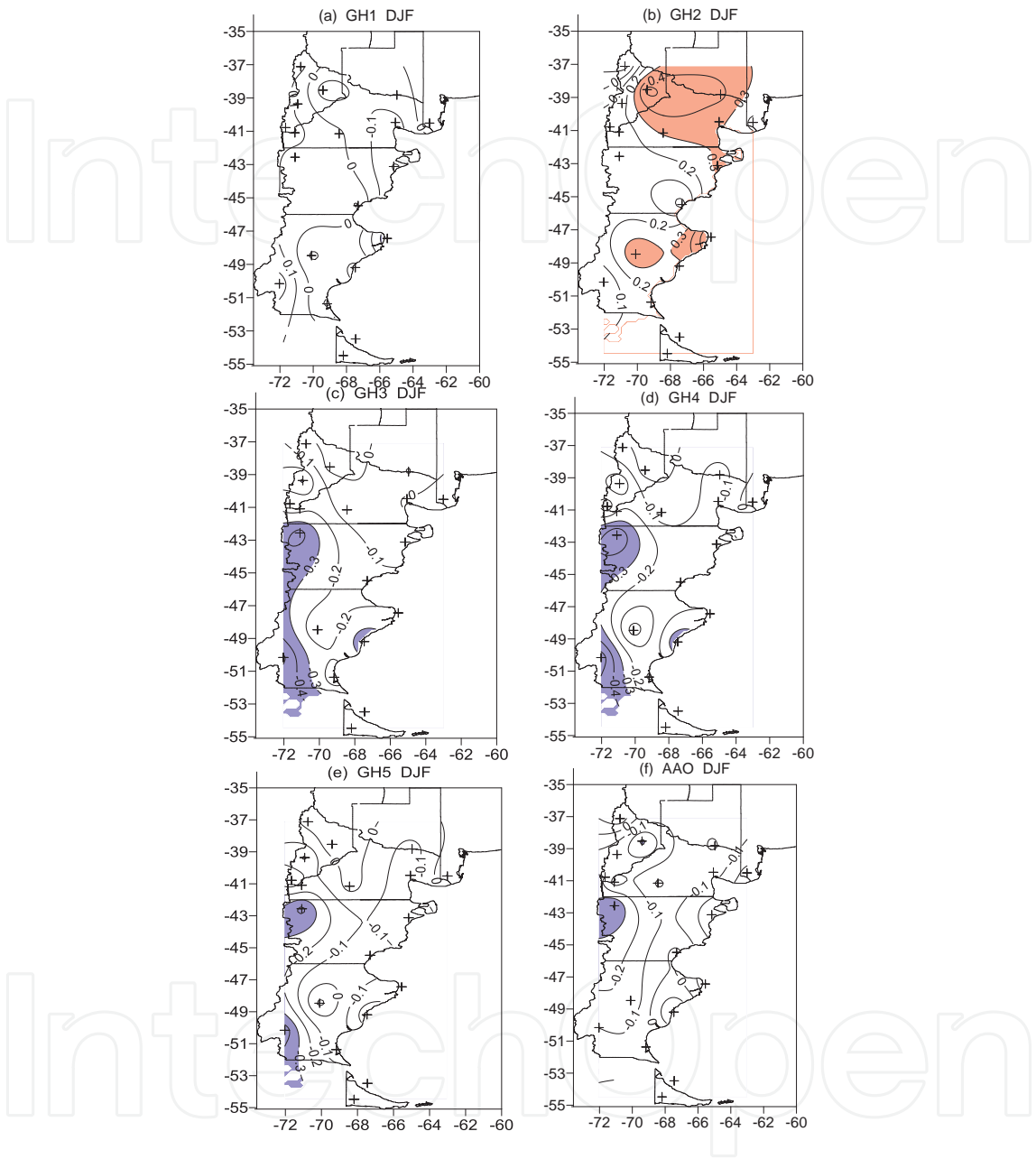
Figure 14. Idem figure 5 for DJF.
