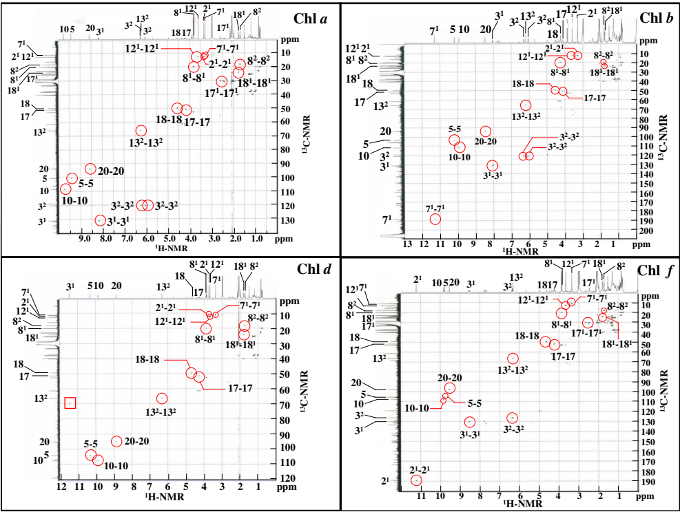
Figure 14. ^1\text{H} - ^{13}\text{C} -HSQC spectra of Chls a , b , d and f measured in acetone- d_6 at 273 K. \square in Chl d : \delta C189.59 (folded from outside the spectral window)
