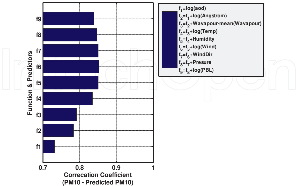
Figure 15. The correlation coefficient between the predicted and measured PM 10 is presented for 8 different models
