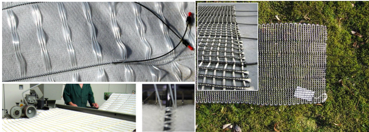
Figure 11. Integration of POF into nonwoven geotextiles at STFI e.V. (left) and a geogrid containing POF (right).
